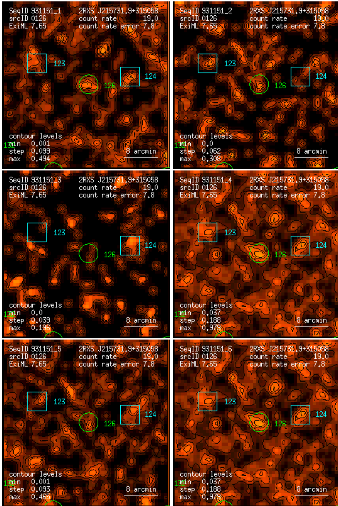
Figure 126: RASS 931151: detection 0126: band rate images, Gaussian filter: (1) PSPC channels 11 – 41, (2) 52 – 90, (3) 91 – 201, (4) 11 – 235, (5) 52 – 201, (6) 11 – 201. Broad band rates in counts/ks. Band rate contour levels in counts/ks/arcmin 2 .
