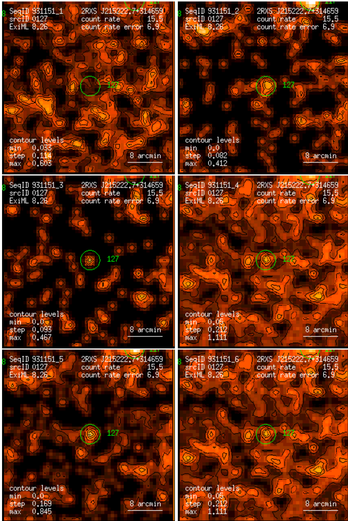
Figure 127: RASS 931151: detection 0127: band rate images, Gaussian filter: (1) PSPC channels 11 – 41, (2) 52 – 90, (3) 91 – 201, (4) 11 – 235, (5) 52 – 201, (6) 11 – 201. Broad band rates in counts/ks. Band rate contour levels in counts/ks/arcmin 2 .
