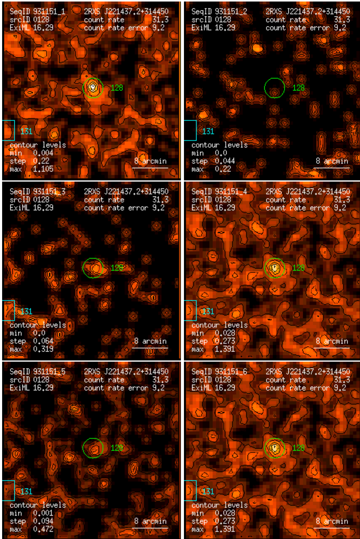
Figure 128: RASS 931151: detection 0128: band rate images, Gaussian filter: (1) PSPC channels 11 – 41, (2) 52 – 90, (3) 91 – 201, (4) 11 – 235, (5) 52 – 201, (6) 11 – 201. Broad band rates in counts/ks. Band rate contour levels in counts/ks/arcmin 2 .
