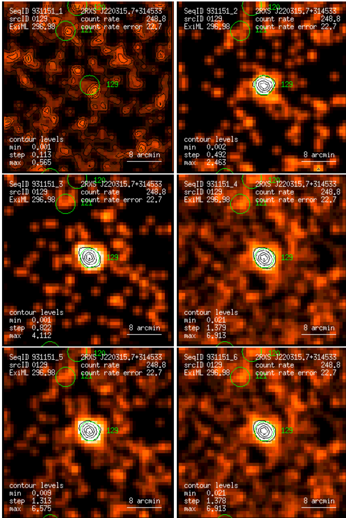
Figure 129: RASS 931151: detection 0129: band rate images, Gaussian filter: (1) PSPC channels 11 – 41, (2) 52 – 90, (3) 91 – 201, (4) 11 – 235, (5) 52 – 201, (6) 11 – 201. Broad band rates in counts/ks. Band rate contour levels in counts/ks/arcmin 2 .
