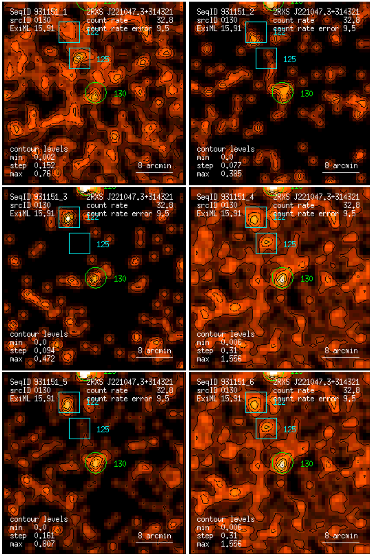
Figure 130: RASS 931151: detection 0130: band rate images, Gaussian filter: (1) PSPC channels 11 – 41, (2) 52 – 90, (3) 91 – 201, (4) 11 – 235, (5) 52 – 201, (6) 11 – 201. Broad band rates in counts/ks. Band rate contour levels in counts/ks/arcmin 2 .
