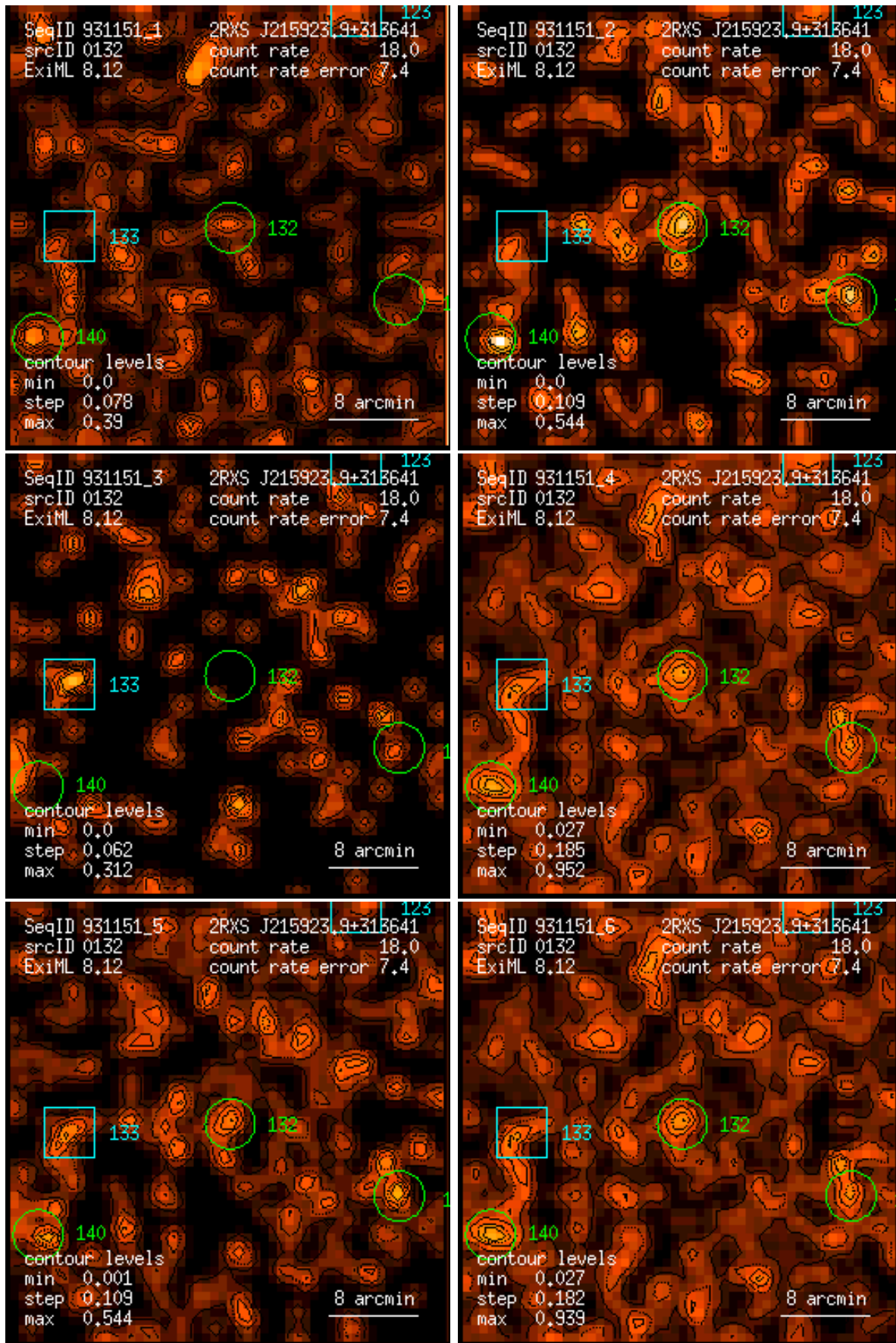
Figure 132: RASS 931151: detection 0132: band rate images, Gaussian filter: (1) PSPC channels 11 – 41, (2) 52 – 90, (3) 91 – 201, (4) 11 – 235, (5) 52 – 201, (6) 11 – 201. Broad band rates in counts/ks. Band rate contour levels in counts/ks/arcmin 2 .
