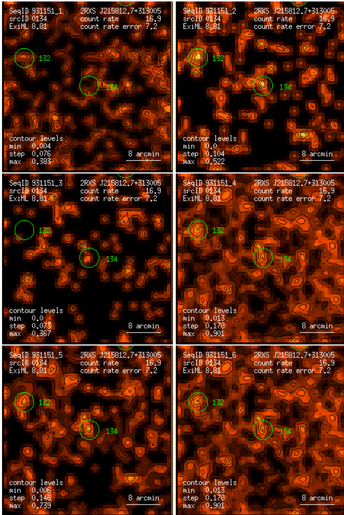
Figure 134: RASS 931151: detection 0134: band rate images, Gaussian filter: (1) PSPC channels 11 – 41, (2) 52 – 90, (3) 91 – 201, (4) 11 – 235, (5) 52 – 201, (6) 11 – 201. Broad band rates in counts/ks. Band rate contour levels in counts/ks/arcmin 2 .
