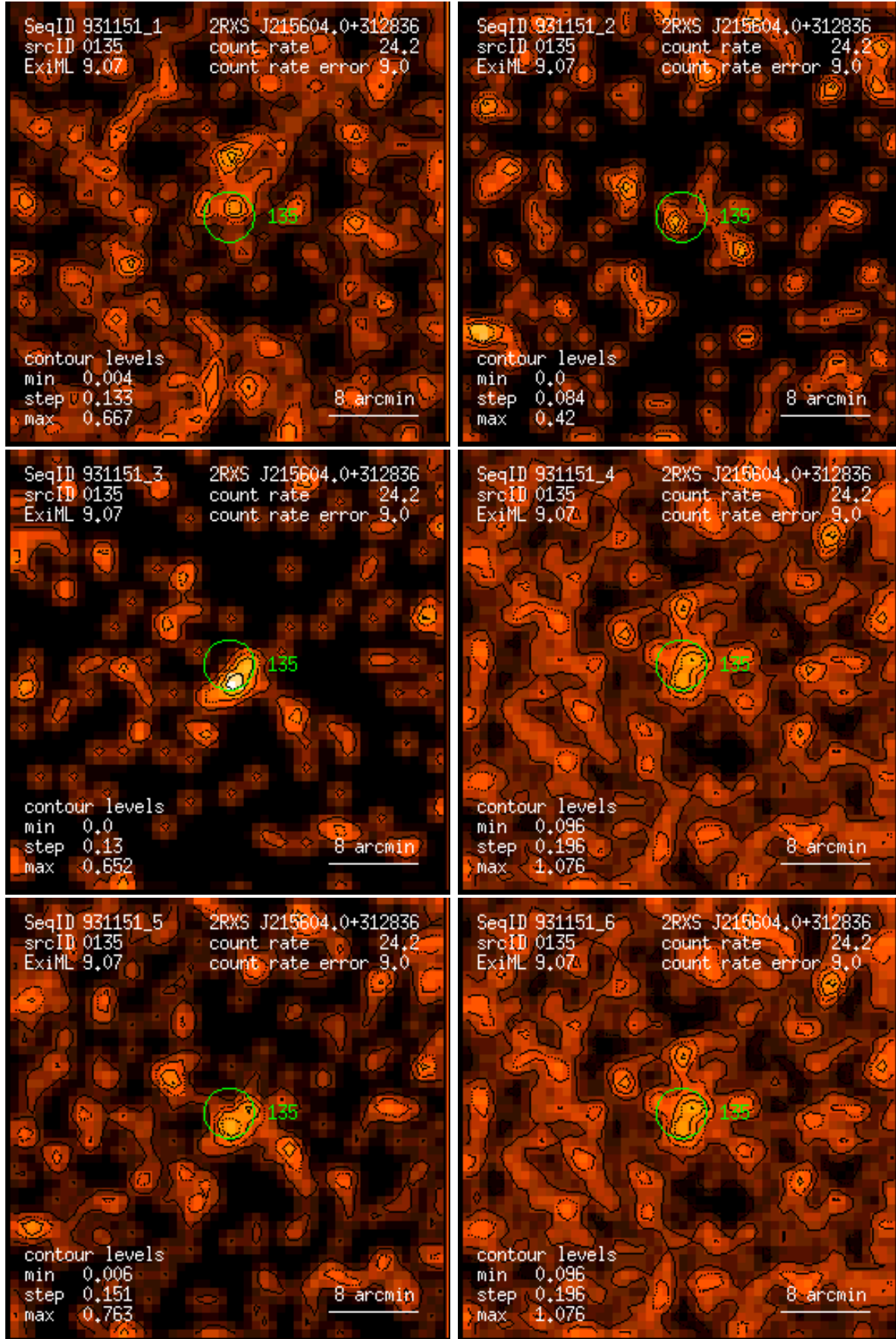
Figure 135: RASS 931151: detection 0135: band rate images, Gaussian filter: (1) PSPC channels 11 – 41, (2) 52 – 90, (3) 91 – 201, (4) 11 – 235, (5) 52 – 201, (6) 11 – 201. Broad band rates in counts/ks. Band rate contour levels in counts/ks/arcmin 2 .
