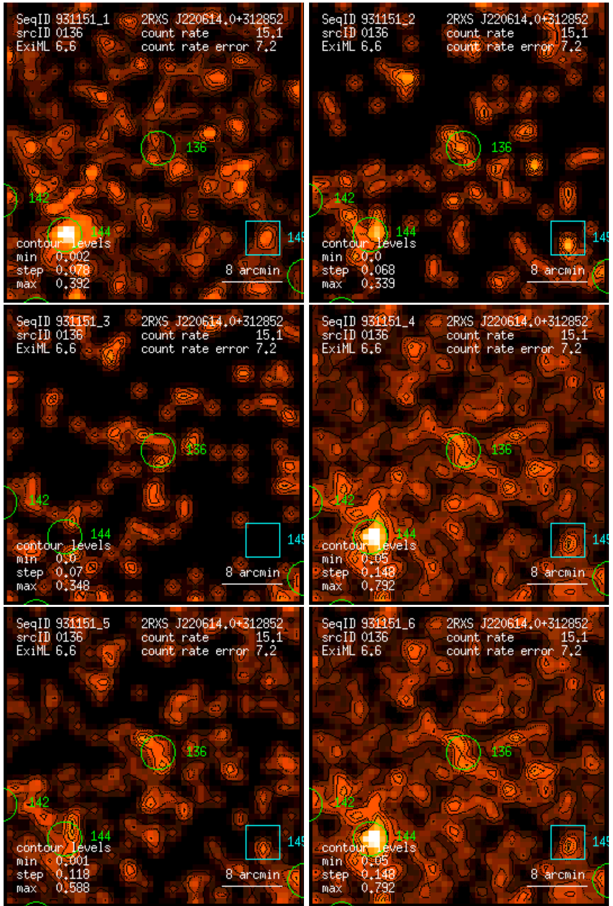
Figure 136: RASS 931151: detection 0136: band rate images, Gaussian filter: (1) PSPC channels 11 – 41, (2) 52 – 90, (3) 91 – 201, (4) 11 – 235, (5) 52 – 201, (6) 11 – 201. Broad band rates in counts/ks. Band rate contour levels in counts/ks/arcmin 2 .
