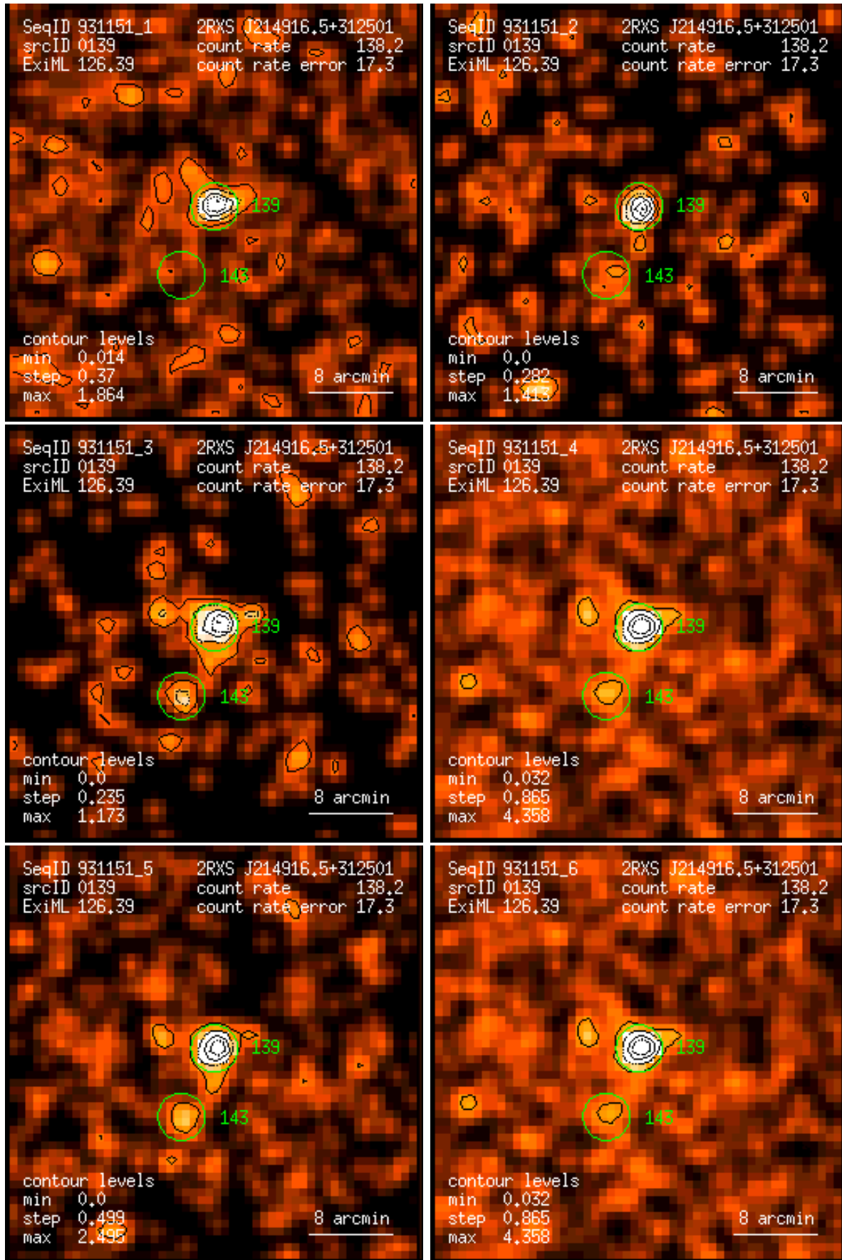
Figure 139: RASS 931151: detection 0139: band rate images, Gaussian filter: (1) PSPC channels 11 – 41, (2) 52 – 90, (3) 91 – 201, (4) 11 – 235, (5) 52 – 201, (6) 11 – 201. Broad band rates in counts/ks. Band rate contour levels in counts/ks/arcmin 2 .
