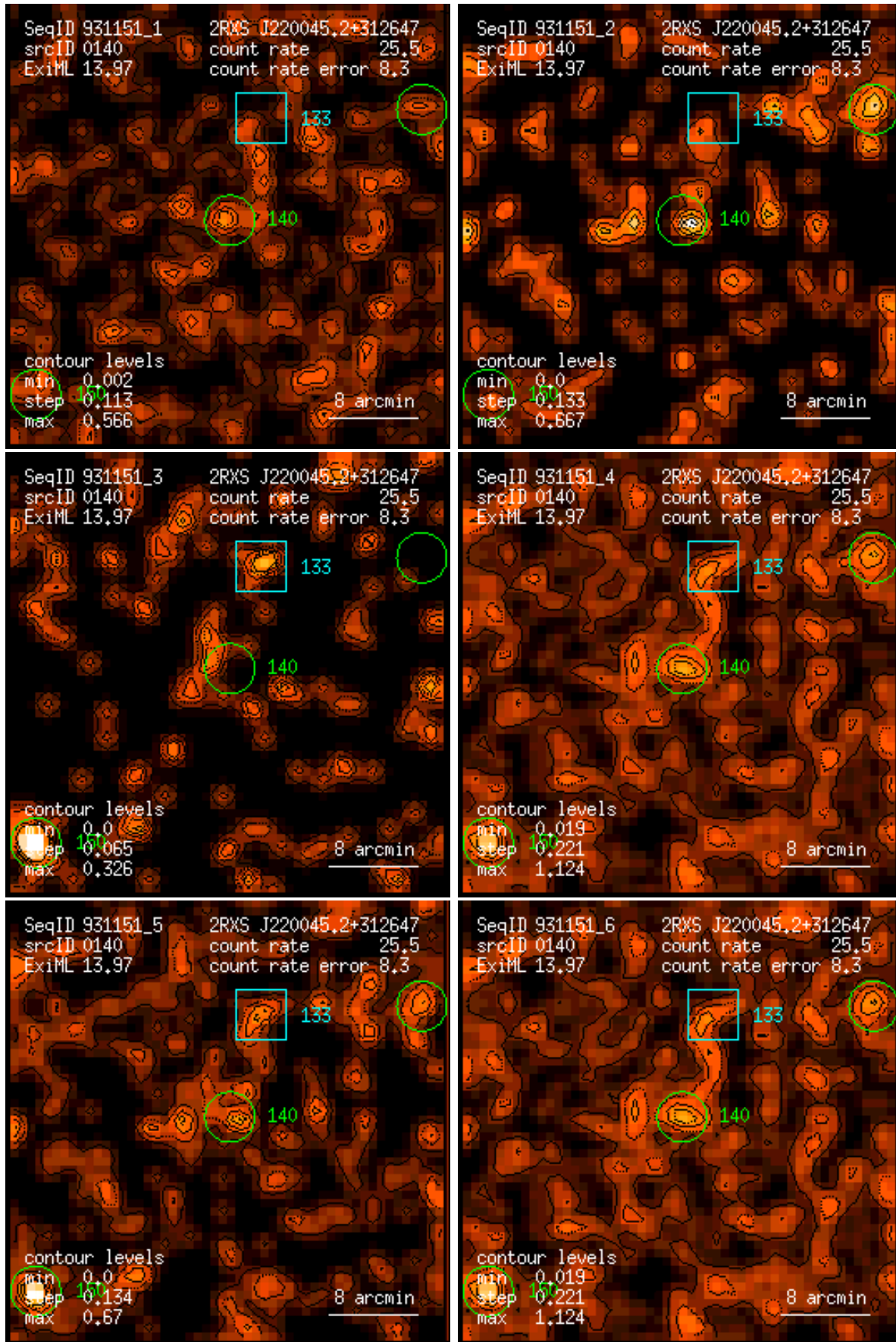
Figure 140: RASS 931151: detection 0140: band rate images, Gaussian filter: (1) PSPC channels 11 – 41, (2) 52 – 90, (3) 91 – 201, (4) 11 – 235, (5) 52 – 201, (6) 11 – 201. Broad band rates in counts/ks. Band rate contour levels in counts/ks/arcmin 2 .
