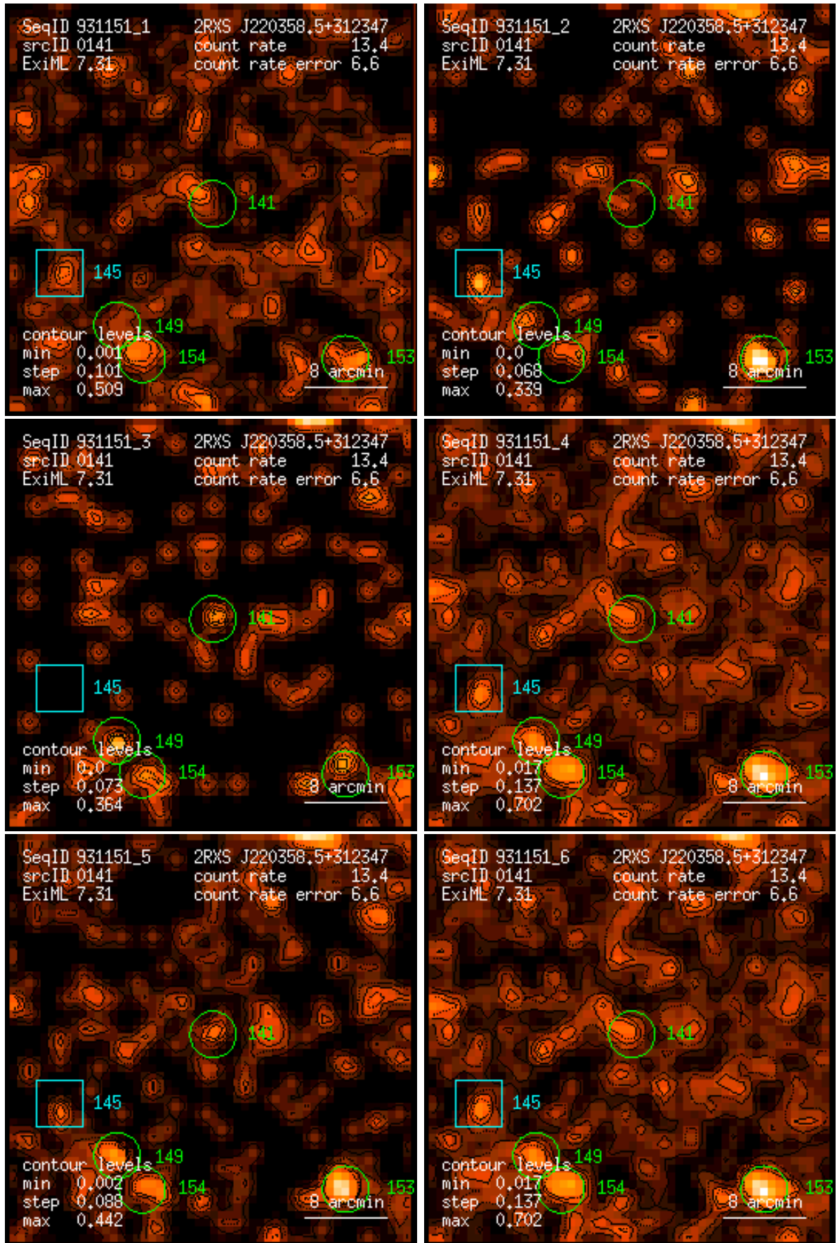
Figure 141: RASS 931151: detection 0141: band rate images, Gaussian filter: (1) PSPC channels 11 – 41, (2) 52 – 90, (3) 91 – 201, (4) 11 – 235, (5) 52 – 201, (6) 11 – 201. Broad band rates in counts/ks. Band rate contour levels in counts/ks/arcmin 2 .
