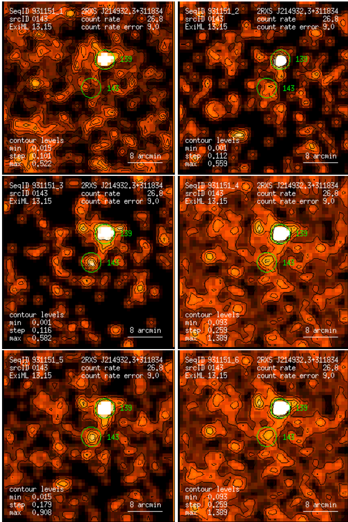
Figure 143: RASS 931151: detection 0143: band rate images, Gaussian filter: (1) PSPC channels 11 – 41, (2) 52 – 90, (3) 91 – 201, (4) 11 – 235, (5) 52 – 201, (6) 11 – 201. Broad band rates in counts/ks. Band rate contour levels in counts/ks/arcmin 2 .
