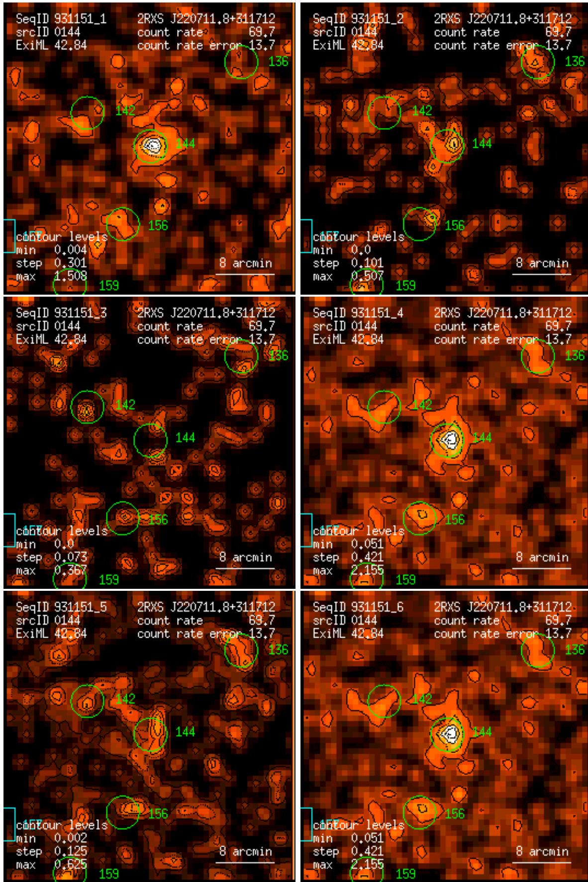
Figure 144: RASS 931151: detection 0144: band rate images, Gaussian filter: (1) PSPC channels 11 – 41, (2) 52 – 90, (3) 91 – 201, (4) 11 – 235, (5) 52 – 201, (6) 11 – 201. Broad band rates in counts/ks. Band rate contour levels in counts/ks/arcmin 2 .
