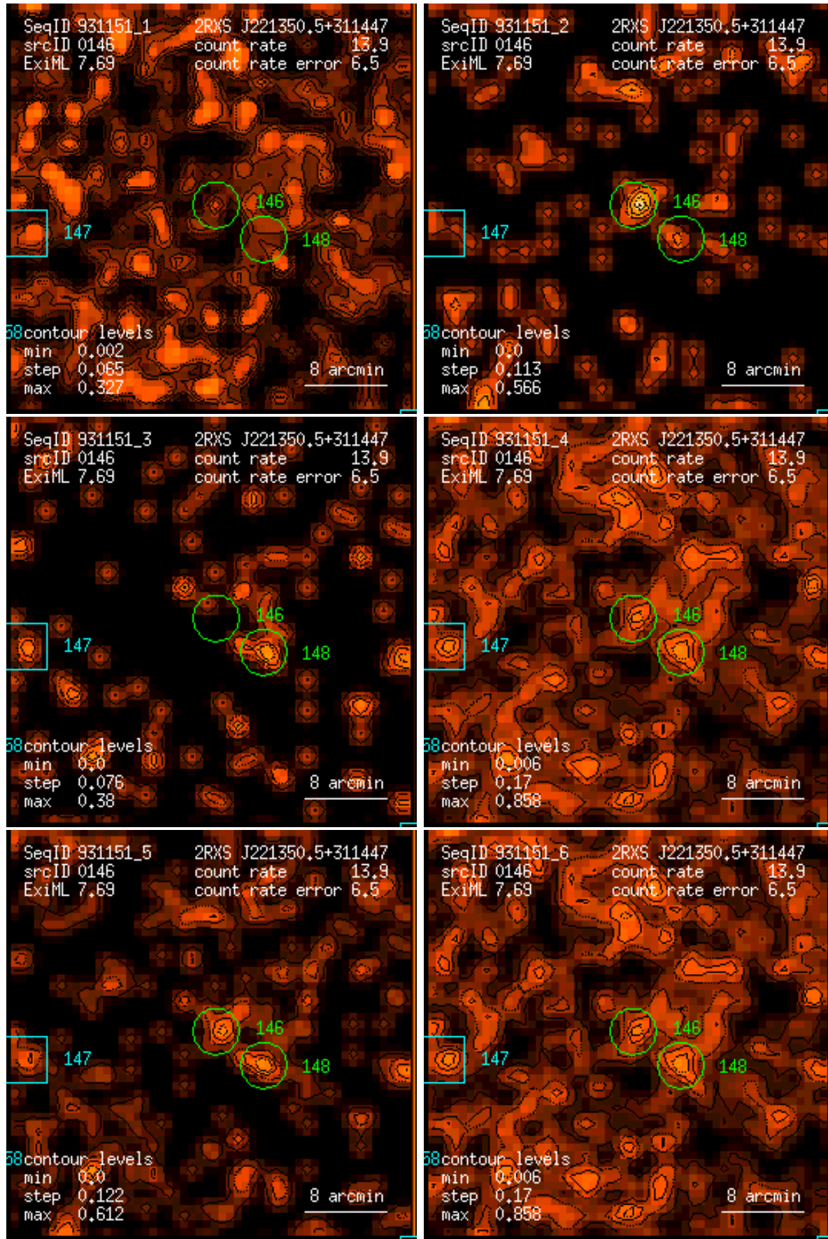
Figure 146: RASS 931151: detection 0146: band rate images, Gaussian filter: (1) PSPC channels 11 – 41, (2) 52 – 90, (3) 91 – 201, (4) 11 – 235, (5) 52 – 201, (6) 11 – 201. Broad band rates in counts/ks. Band rate contour levels in counts/ks/arcmin 2 .
