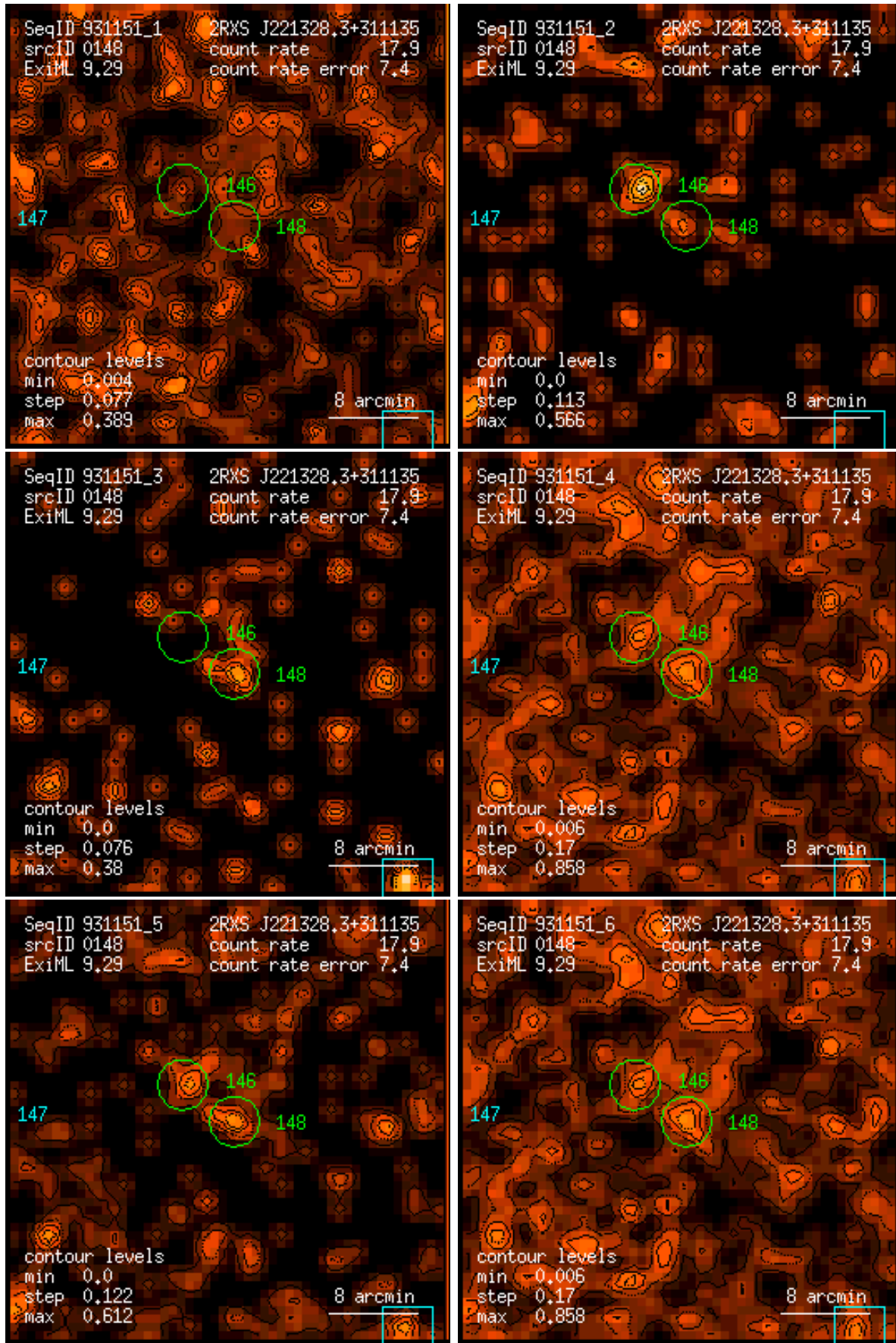
Figure 148: RASS 931151: detection 0148: band rate images, Gaussian filter: (1) PSPC channels 11 – 41, (2) 52 – 90, (3) 91 – 201, (4) 11 – 235, (5) 52 – 201, (6) 11 – 201. Broad band rates in counts/ks. Band rate contour levels in counts/ks/arcmin 2 .
