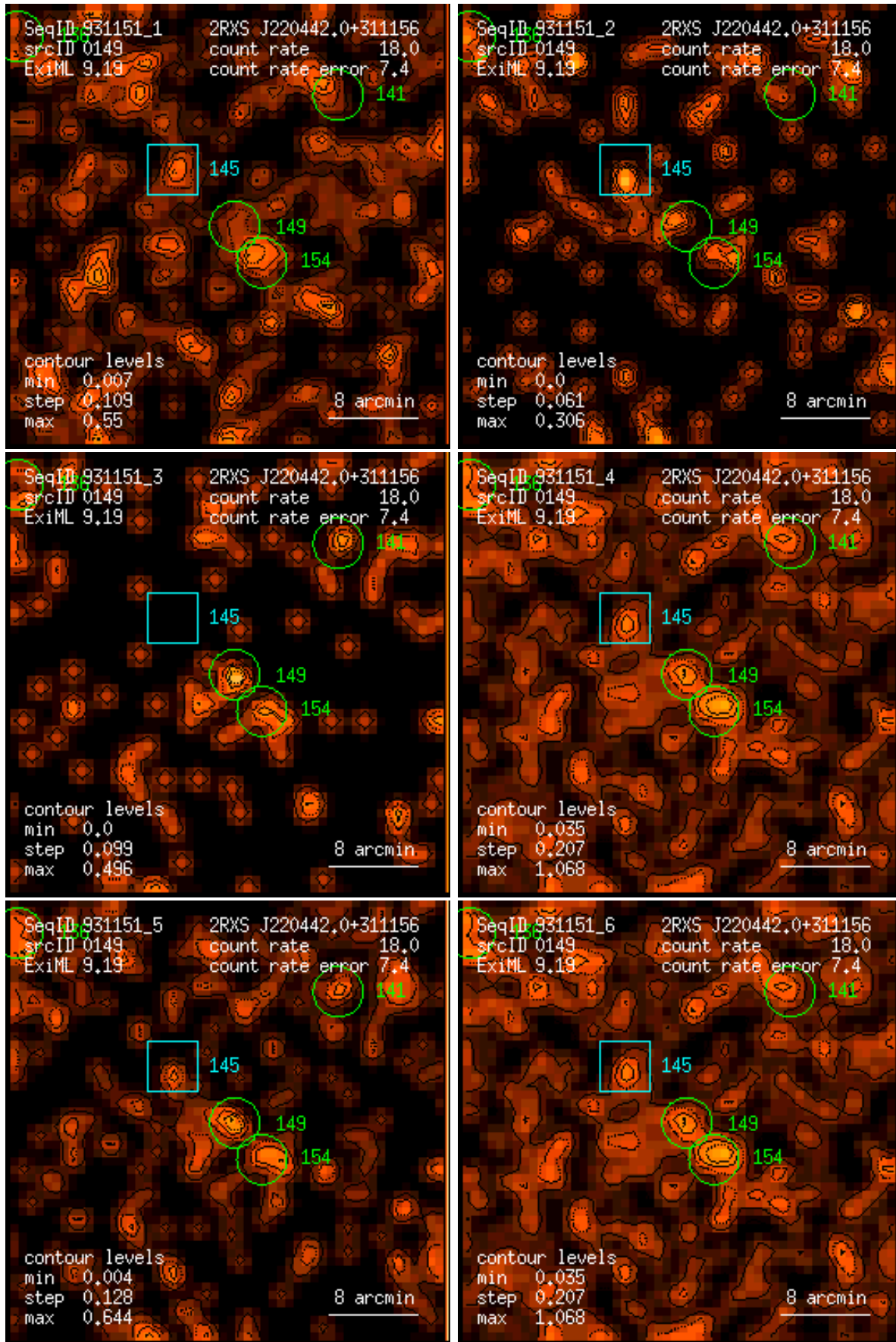
Figure 149: RASS 931151: detection 0149: band rate images, Gaussian filter: (1) PSPC channels 11 – 41, (2) 52 – 90, (3) 91 – 201, (4) 11 – 235, (5) 52 – 201, (6) 11 – 201. Broad band rates in counts/ks. Band rate contour levels in counts/ks/arcmin 2 .
