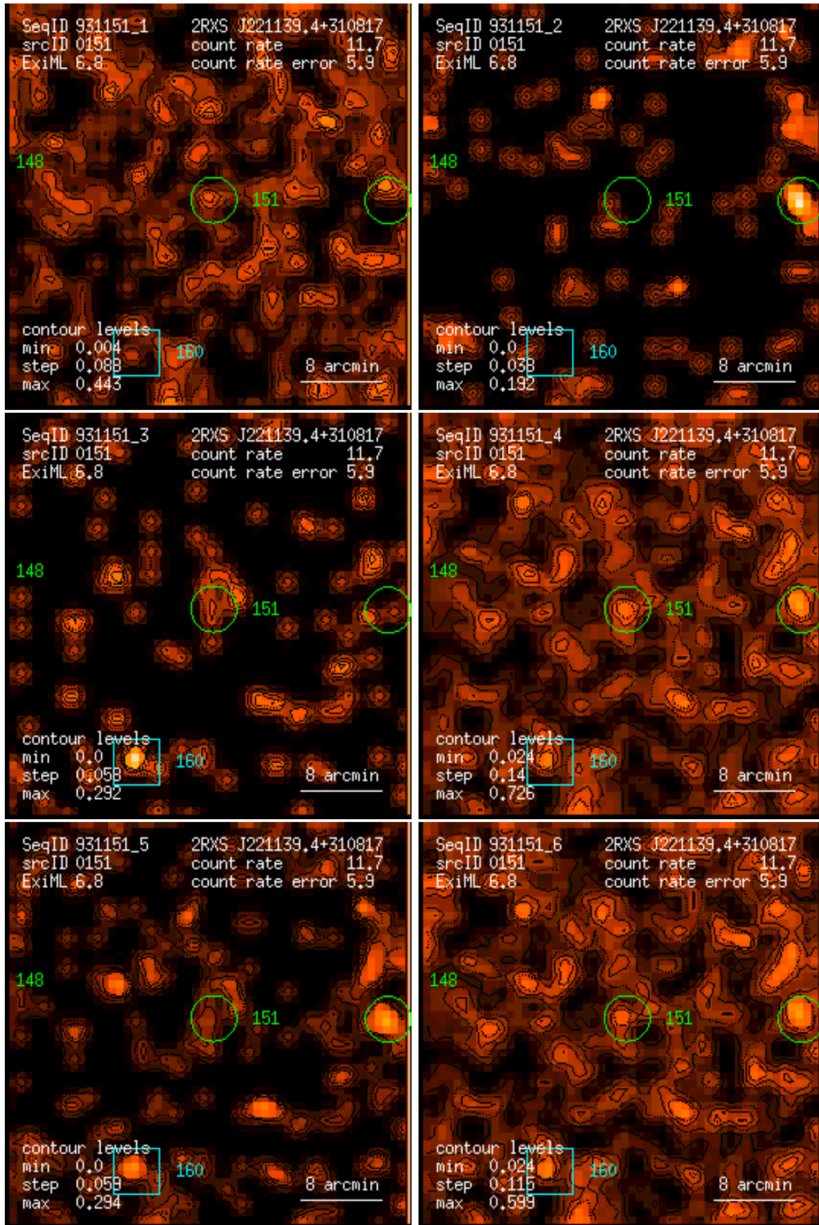
Figure 151: RASS 931151: detection 0151: band rate images, Gaussian filter: (1) PSPC channels 11 – 41, (2) 52 – 90, (3) 91 – 201, (4) 11 – 235, (5) 52 – 201, (6) 11 – 201. Broad band rates in counts/ks. Band rate contour levels in counts/ks/arcmin 2 .
