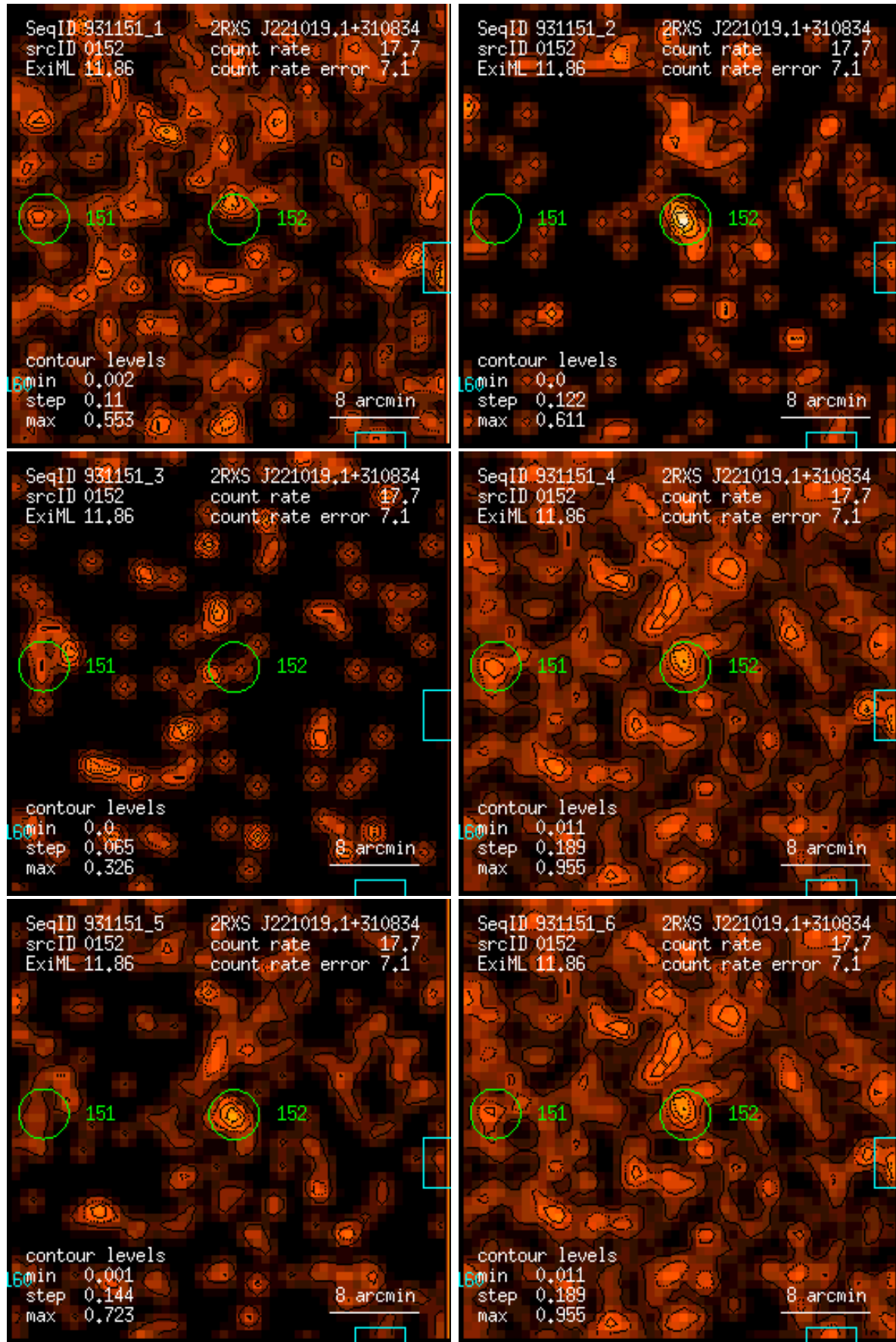
Figure 152: RASS 931151: detection 0152: band rate images, Gaussian filter: (1) PSPC channels 11 – 41, (2) 52 – 90, (3) 91 – 201, (4) 11 – 235, (5) 52 – 201, (6) 11 – 201. Broad band rates in counts/ks. Band rate contour levels in counts/ks/arcmin 2 .
