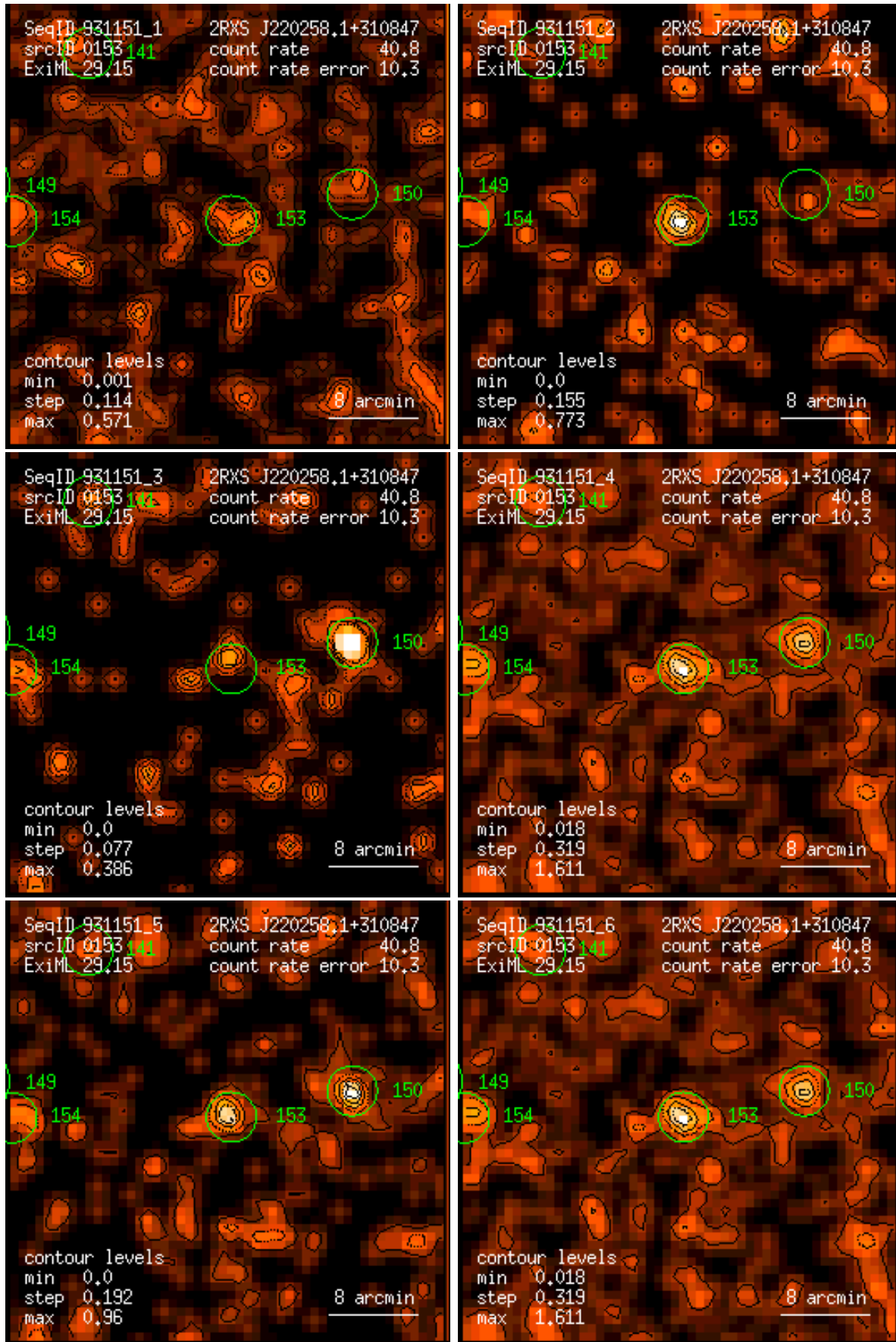
Figure 153: RASS 931151: detection 0153: band rate images, Gaussian filter: (1) PSPC channels 11 – 41, (2) 52 – 90, (3) 91 – 201, (4) 11 – 235, (5) 52 – 201, (6) 11 – 201. Broad band rates in counts/ks. Band rate contour levels in counts/ks/arcmin 2 .
