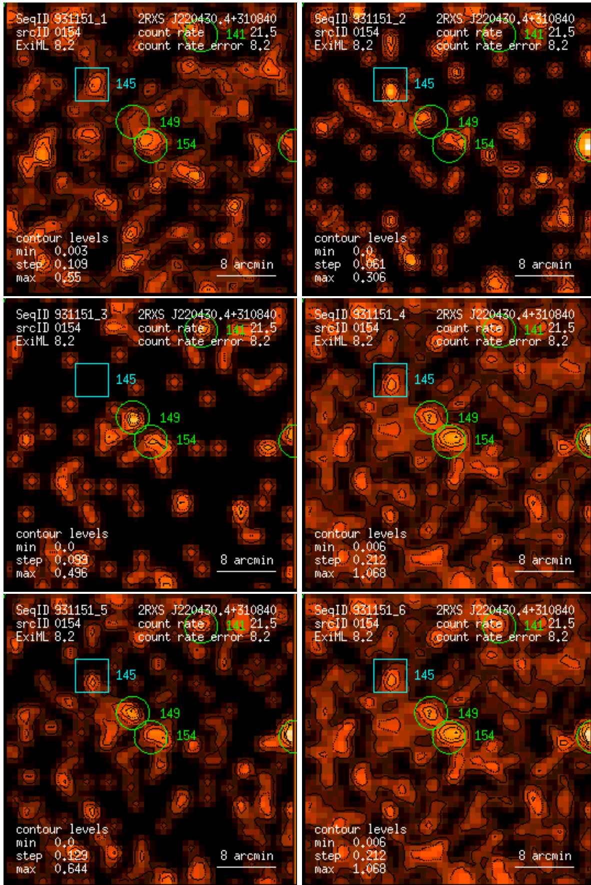
Figure 154: RASS 931151: detection 0154: band rate images, Gaussian filter: (1) PSPC channels 11 – 41, (2) 52 – 90, (3) 91 – 201, (4) 11 – 235, (5) 52 – 201, (6) 11 – 201. Broad band rates in counts/ks. Band rate contour levels in counts/ks/arcmin 2 .
