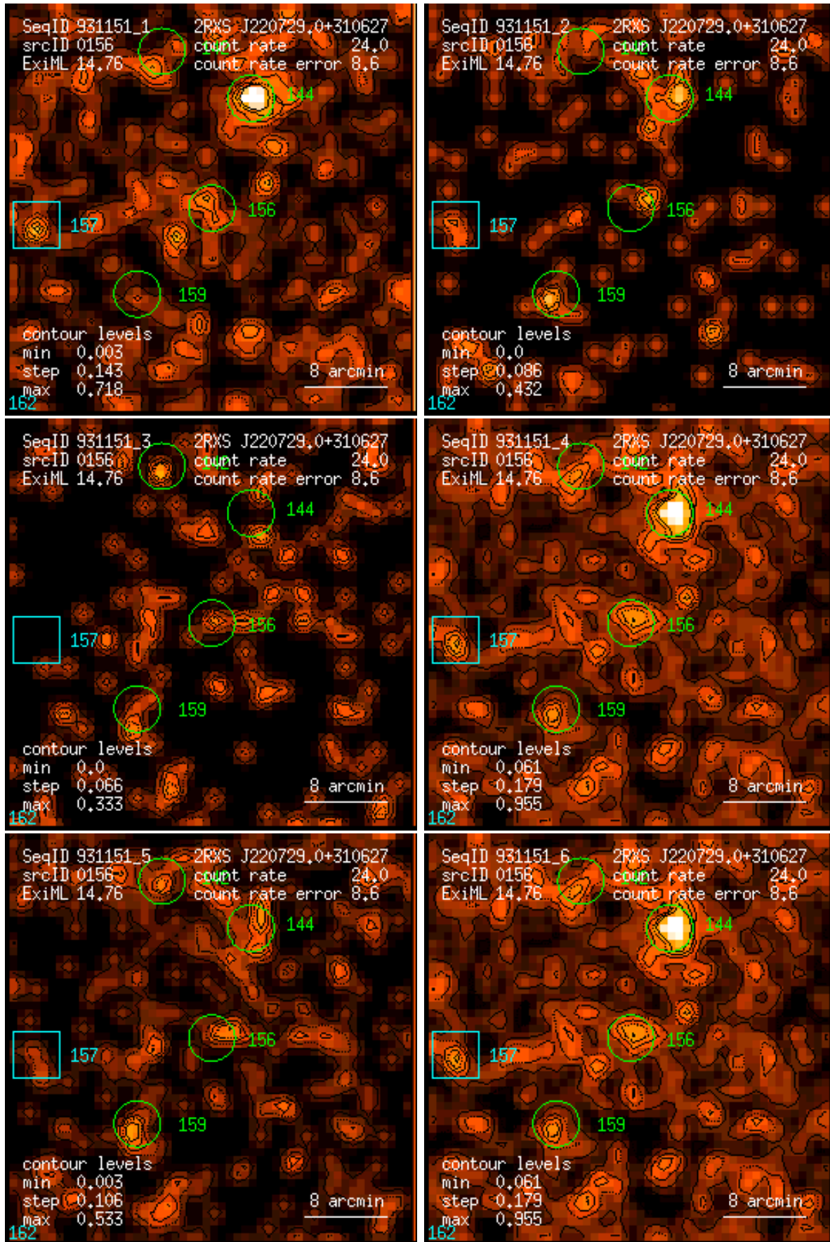
Figure 156: RASS 931151: detection 0156: band rate images, Gaussian filter: (1) PSPPC channels 11 – 41, (2) 52 – 90, (3) 91 – 201, (4) 11 – 235, (5) 52 – 201, (6) 11 – 201. Broad band rates in counts/ks. Band rate contour levels in counts/ks/arcmin 2 .
