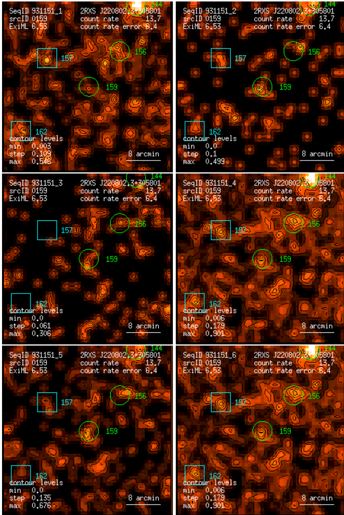
Figure 159: RASS 931151: detection 0159: band rate images, Gaussian filter: (1) PSPC channels 11 – 41, (2) 52 – 90, (3) 91 – 201, (4) 11 – 235, (5) 52 – 201, (6) 11 – 201. Broad band rates in counts/ks. Band rate contour levels in counts/ks/arcmin 2 .
