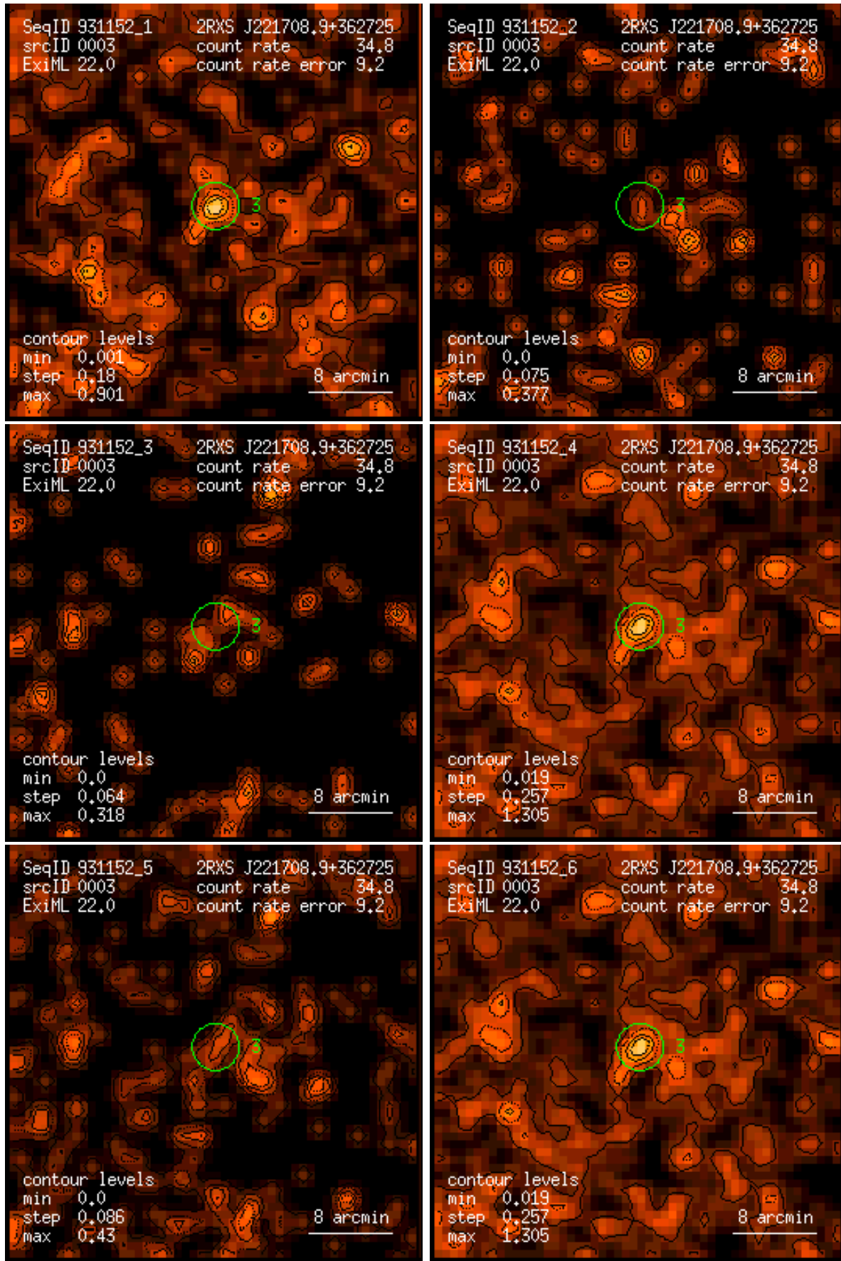
Figure 3: RASS 931152: detection 0003: band rate images, Gaussian filter: (1) PSPC channels 11 – 41, (2) 52 – 90, (3) 91 – 201, (4) 11 – 235, (5) 52 – 201, (6) 11 – 201. Broad band rates in counts/ks. Band rate contour levels in counts/ks/arcmin 2 .
