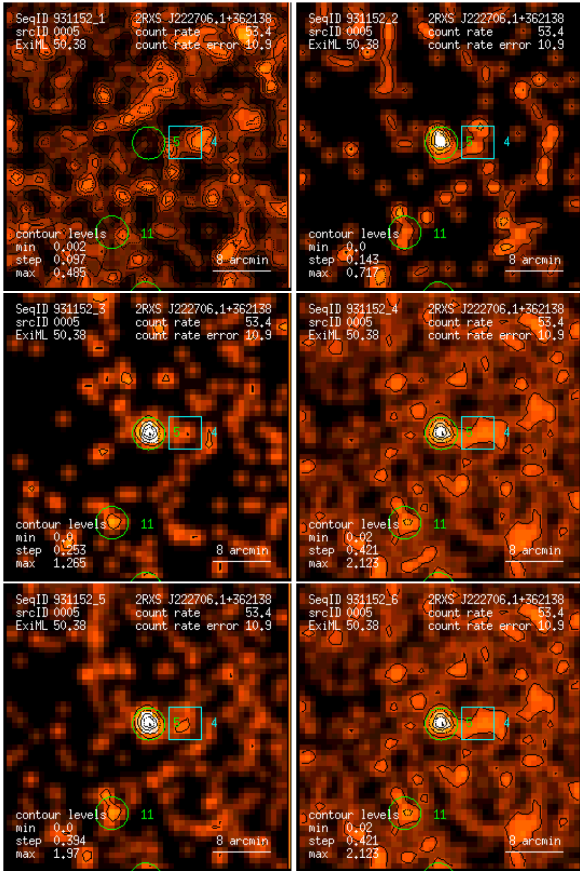
Figure 5: RASS 931152: detection 0005: band rate images, Gaussian filter: (1) PSPC channels 11 – 41, (2) 52 – 90, (3) 91 – 201, (4) 11 – 235, (5) 52 – 201, (6) 11 – 201. Broad band rates in counts/ks. Band rate contour levels in counts/ks/arcmin 2 .
