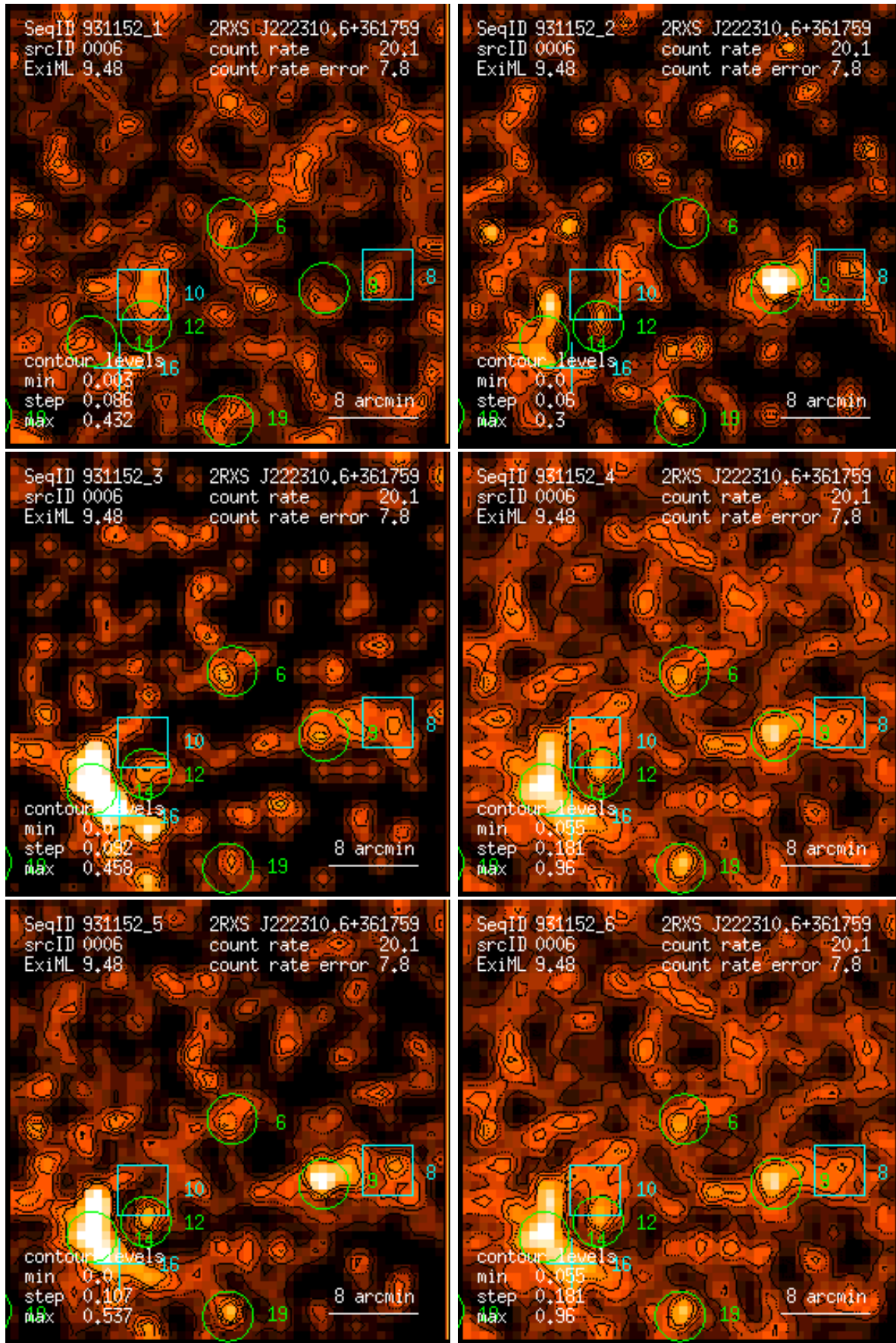
Figure 6: RASS 931152: detection 0006: band rate images, Gaussian filter: (1) PSPC channels 11 – 41, (2) 52 – 90, (3) 91 – 201, (4) 11 – 235, (5) 52 – 201, (6) 11 – 201. Broad band rates in counts/ks. Band rate contour levels in counts/ks/arcmin 2 .
