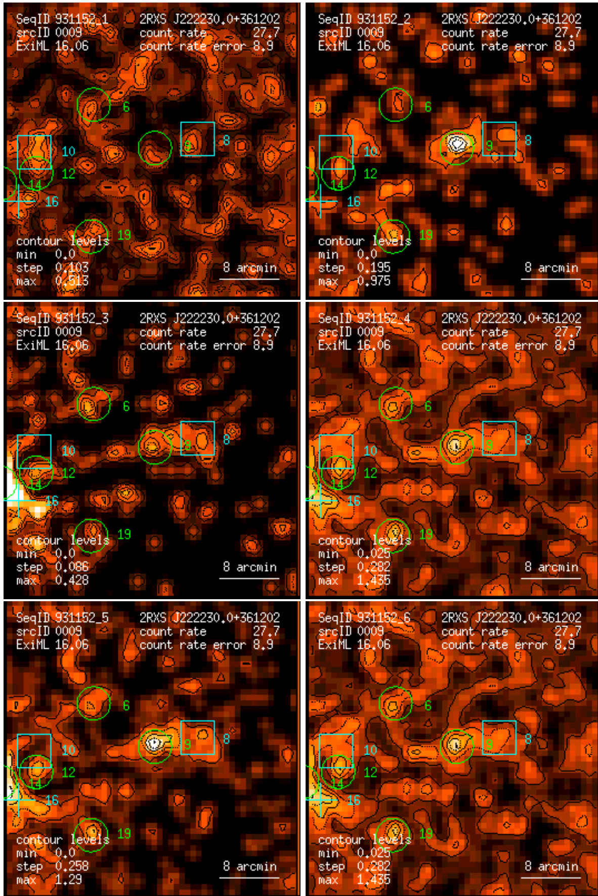
Figure 9: RASS 931152: detection 0009: band rate images, Gaussian filter: (1) PSPC channels 11 – 41, (2) 52 – 90, (3) 91 – 201, (4) 11 – 235, (5) 52 – 201, (6) 11 – 201. Broad band rates in counts/ks. Band rate contour levels in counts/ks/arcmin 2 .
