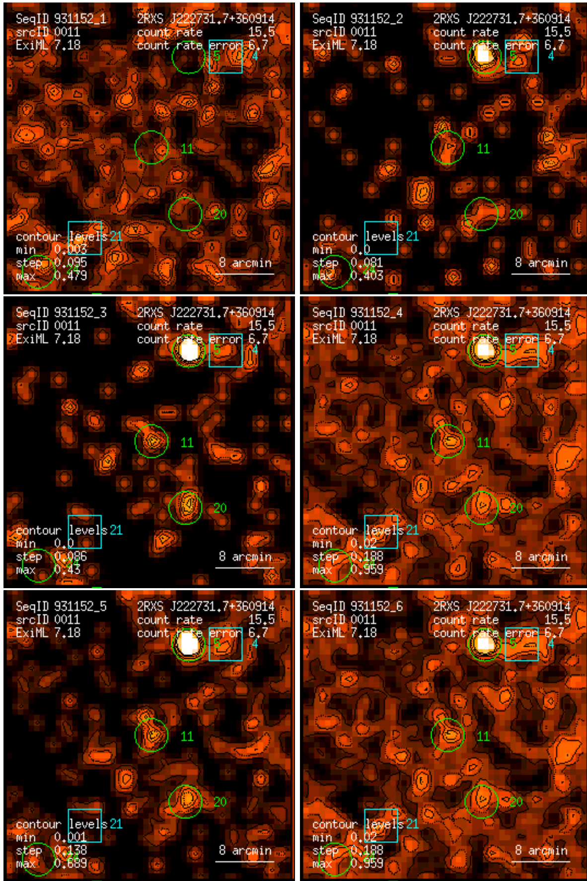
Figure 11: RASS 931152: detection 0011: band rate images, Gaussian filter: (1) PSPC channels 11 – 41, (2) 52 – 90, (3) 91 – 201, (4) 11 – 235, (5) 52 – 201, (6) 11 – 201. Broad band rates in counts/ks. Band rate contour levels in counts/ks/arcmin 2 .
