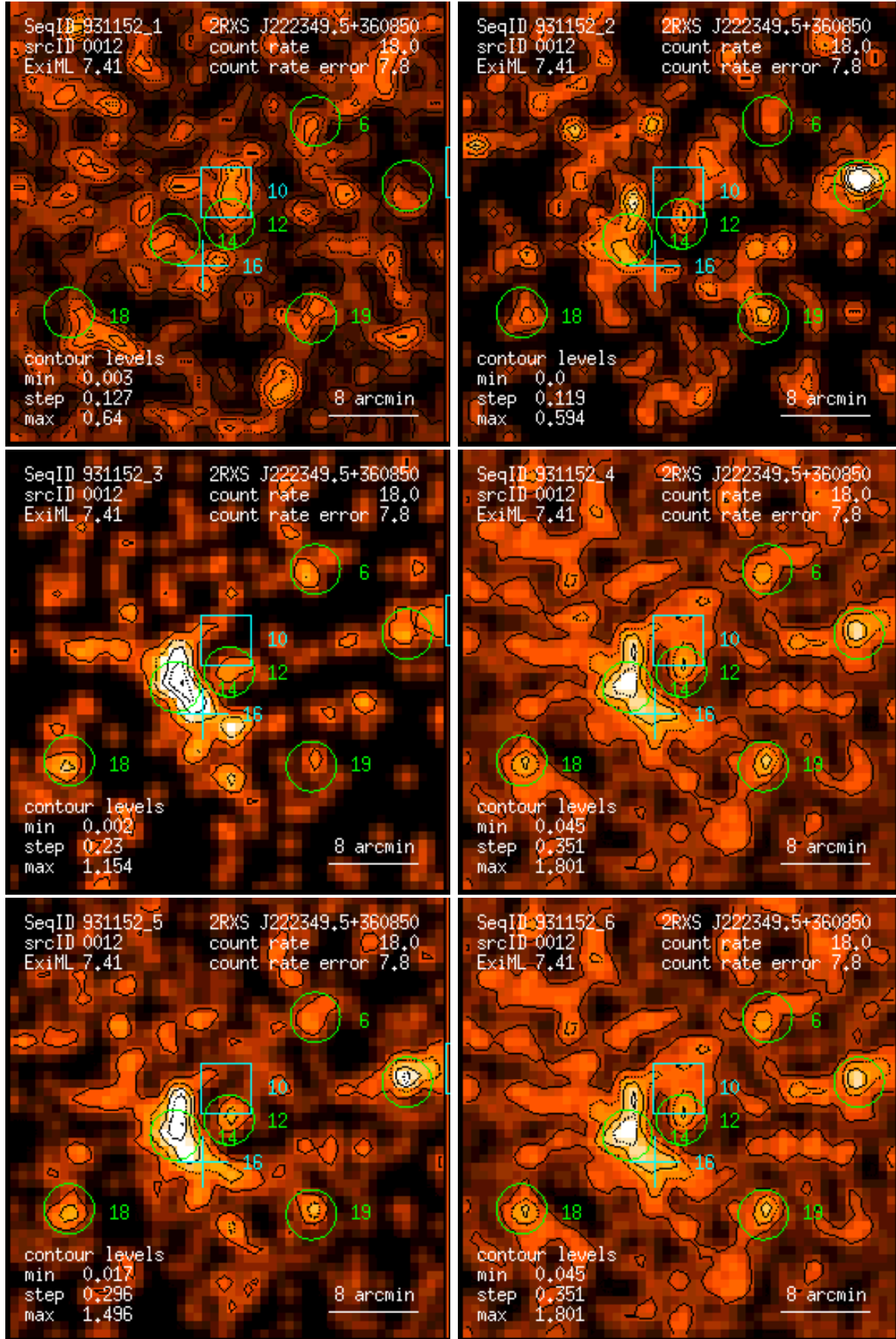
Figure 12: RASS 931152: detection 0012: band rate images, Gaussian filter: (1) PSPC channels 11 – 41, (2) 52 – 90, (3) 91 – 201, (4) 11 – 235, (5) 52 – 201, (6) 11 – 201. Broad band rates in counts/ks. Band rate contour levels in counts/ks/arcmin 2 .
