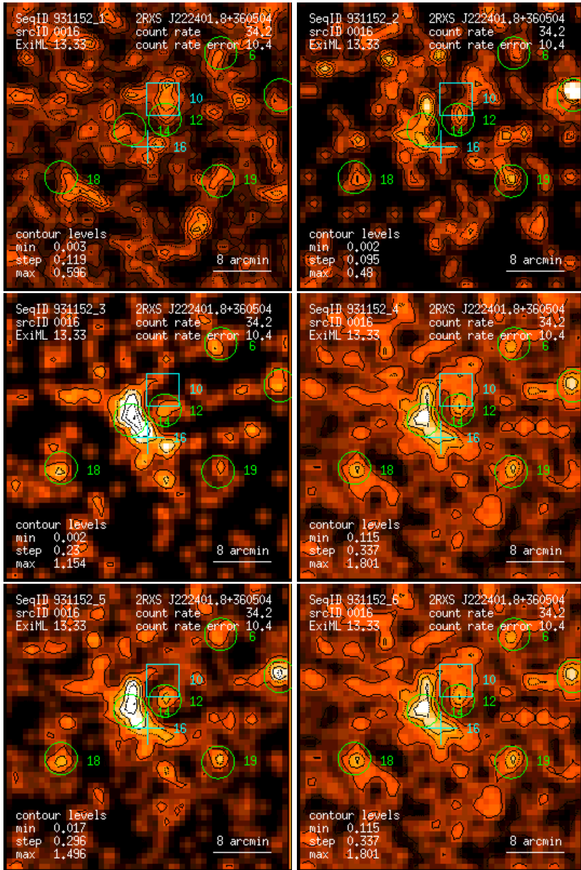
Figure 16: RASS 931152: detection 0016: band rate images, Gaussian filter: (1) PSPC channels 11 – 41, (2) 52 – 90, (3) 91 – 201, (4) 11 – 235, (5) 52 – 201, (6) 11 – 201. Broad band rates in counts/ks. Band rate contour levels in counts/ks/arcmin 2 .
