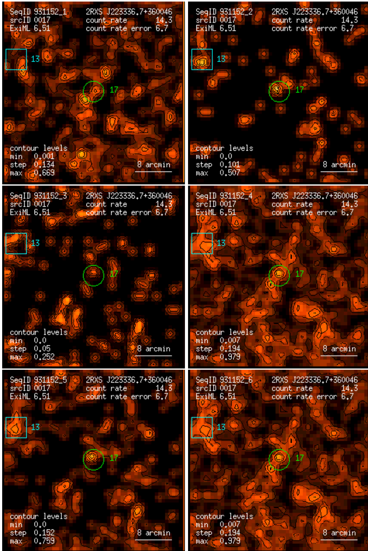
Figure 17: RASS 931152: detection 0017: band rate images, Gaussian filter: (1) PSPC channels 11 – 41, (2) 52 – 90, (3) 91 – 201, (4) 11 – 235, (5) 52 – 201, (6) 11 – 201. Broad band rates in counts/ks. Band rate contour levels in counts/ks/arcmin 2 .
