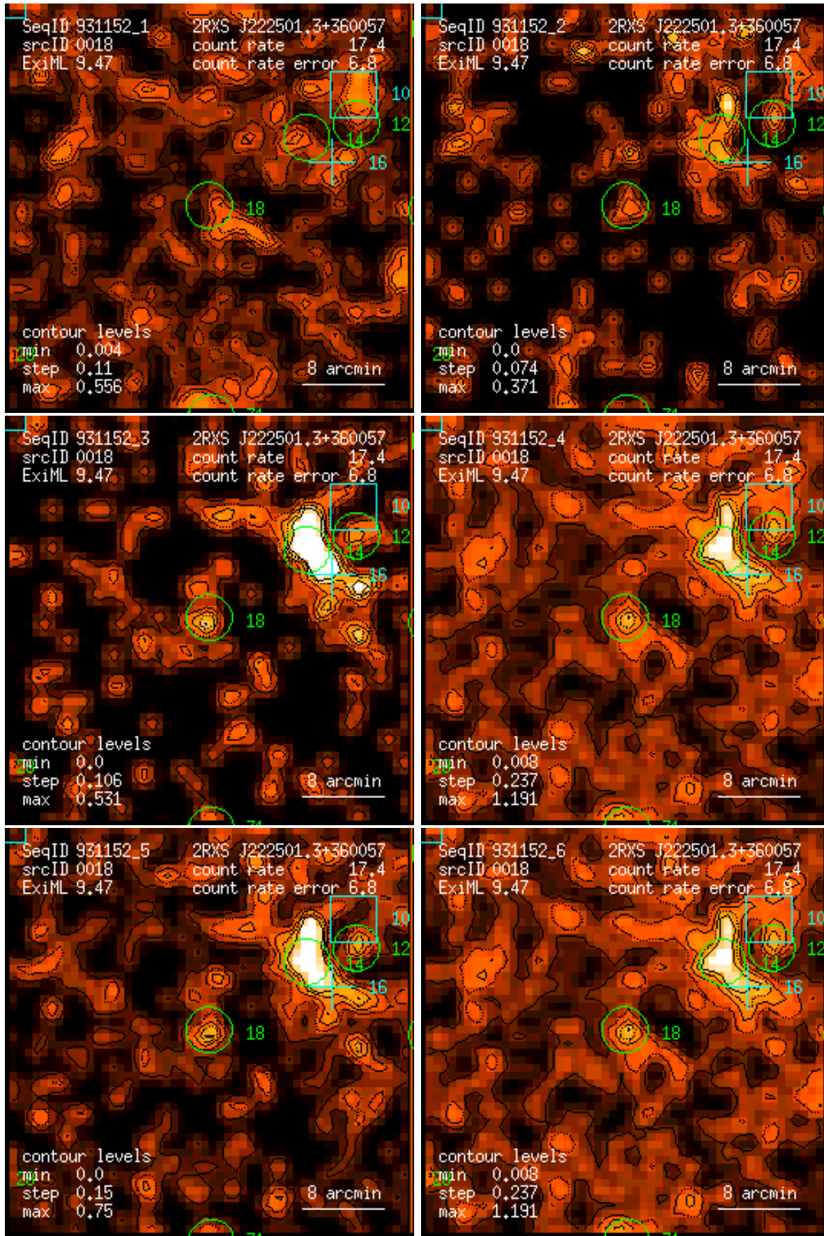
Figure 18: RASS 931152: detection 0018: band rate images, Gaussian filter: (1) PSPC channels 11 – 41, (2) 52 – 90, (3) 91 – 201, (4) 11 – 235, (5) 52 – 201, (6) 11 – 201. Broad band rates in counts/ks. Band rate contour levels in counts/ks/arcmin 2 .
