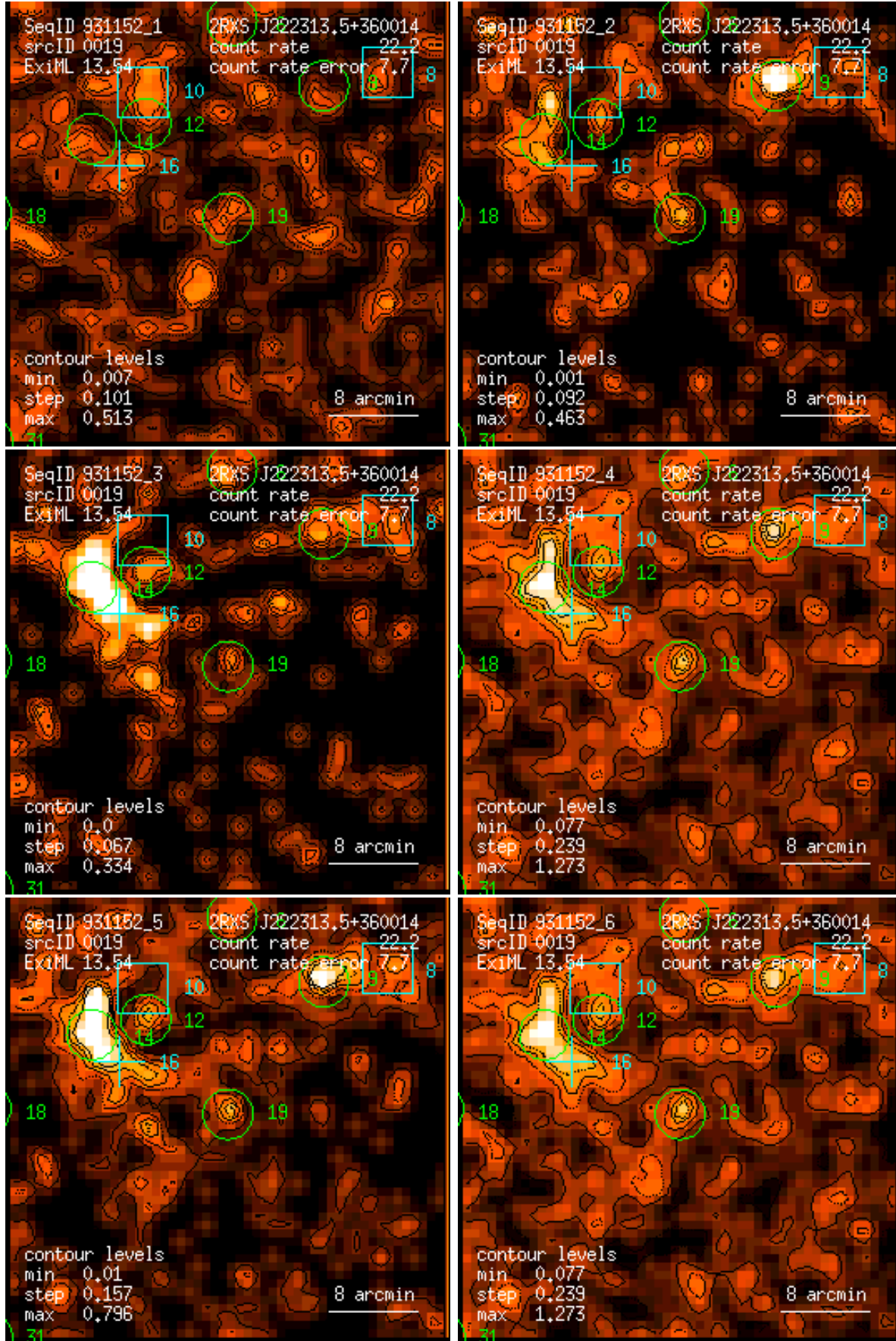
Figure 19: RASS 931152: detection 0019: band rate images, Gaussian filter: (1) PSPC channels 11 – 41, (2) 52 – 90, (3) 91 – 201, (4) 11 – 235, (5) 52 – 201, (6) 11 – 201. Broad band rates in counts/ks. Band rate contour levels in counts/ks/arcmin 2 .
