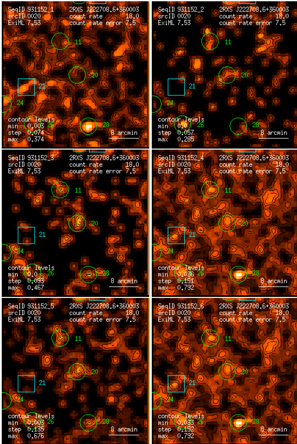
Figure 20: RASS 931152: detection 0020: band rate images, Gaussian filter: (1) PSPC channels 11 – 41, (2) 52 – 90, (3) 91 – 201, (4) 11 – 235, (5) 52 – 201, (6) 11 – 201. Broad band rates in counts/ks. Band rate contour levels in counts/ks/arcmin 2 .
