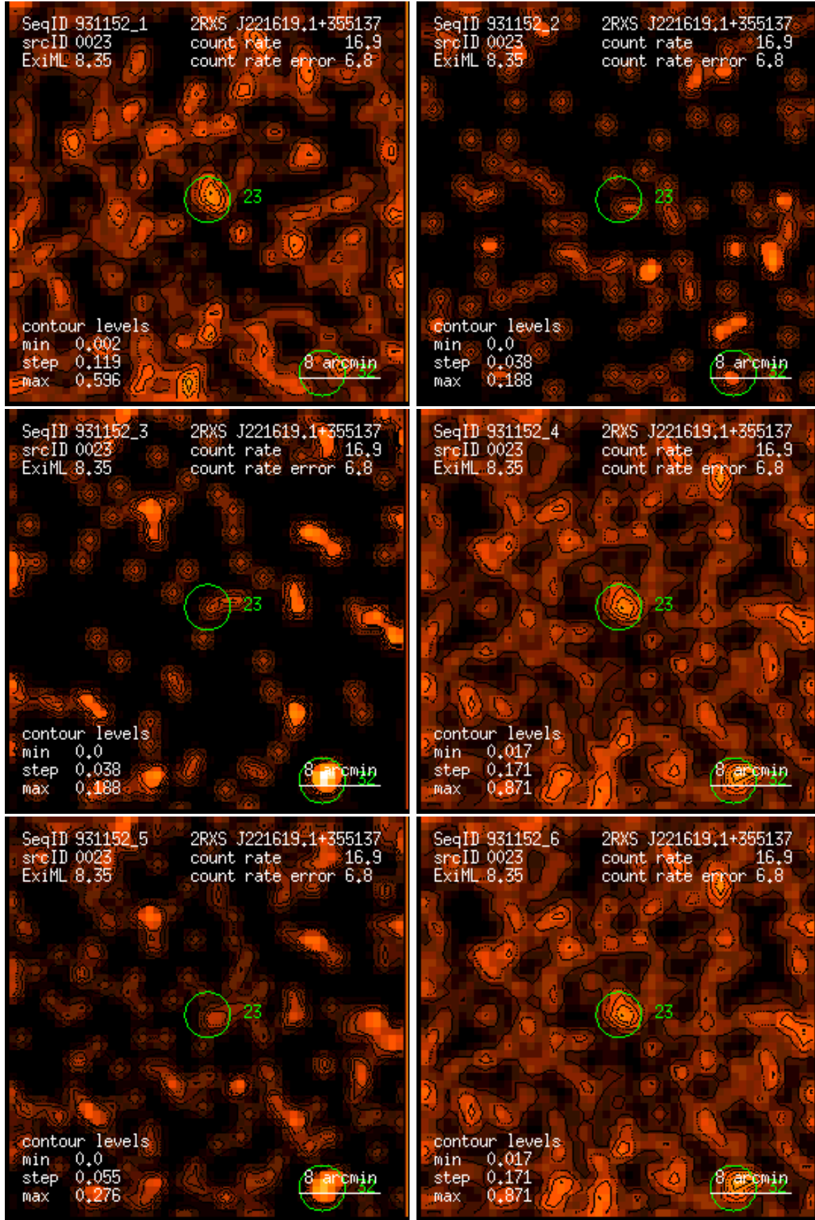
Figure 23: RASS 931152: detection 0023: band rate images, Gaussian filter: (1) PSPC channels 11 – 41, (2) 52 – 90, (3) 91 – 201, (4) 11 – 235, (5) 52 – 201, (6) 11 – 201. Broad band rates in counts/ks. Band rate contour levels in counts/ks/arcmin 2 .
