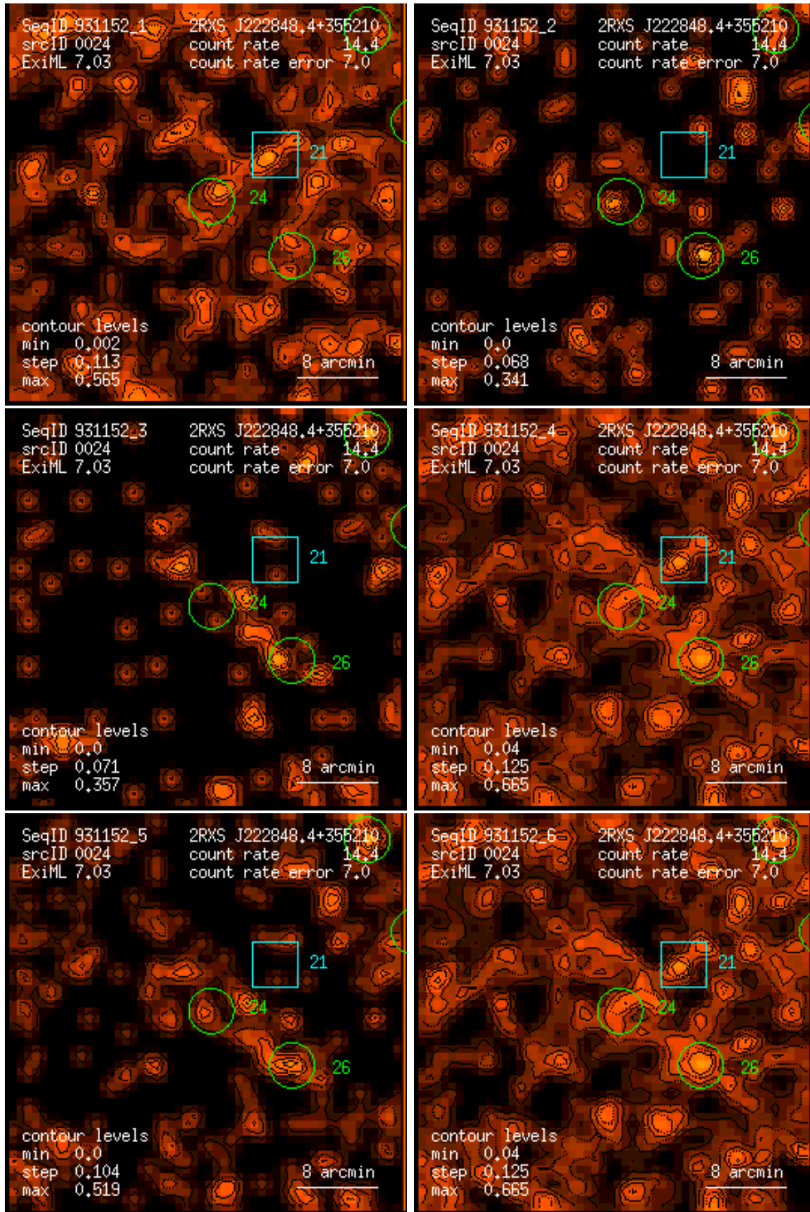
Figure 24: RASS 931152: detection 0024: band rate images, Gaussian filter: (1) PSPC channels 11 – 41, (2) 52 – 90, (3) 91 – 201, (4) 11 – 235, (5) 52 – 201, (6) 11 – 201. Broad band rates in counts/ks. Band rate contour levels in counts/ks/arcmin 2 .
