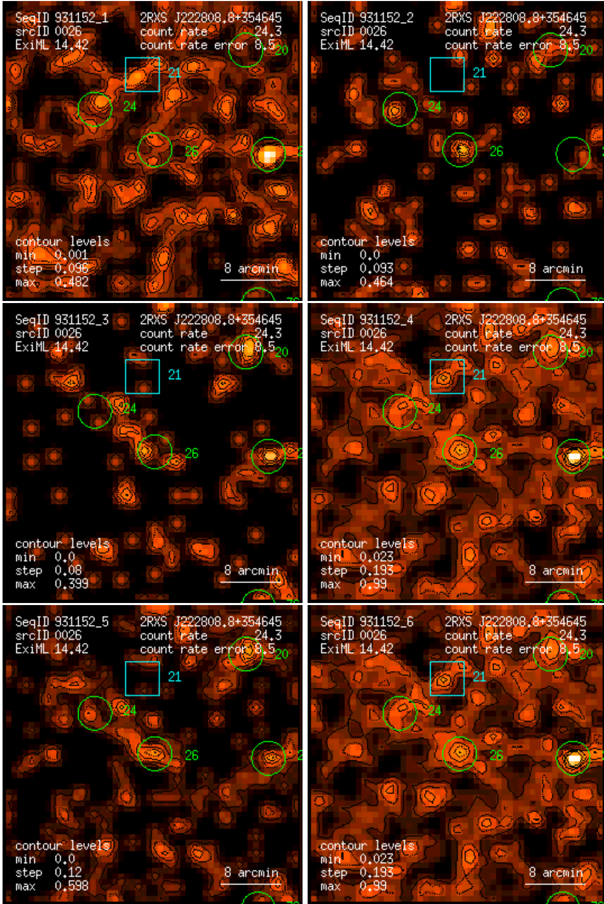
Figure 26: RASS 931152: detection 0026: band rate images, Gaussian filter: (1) PSPC channels 11 – 41, (2) 52 – 90, (3) 91 – 201, (4) 11 – 235, (5) 52 – 201, (6) 11 – 201. Broad band rates in counts/ks. Band rate contour levels in counts/ks/arcmin 2 .
