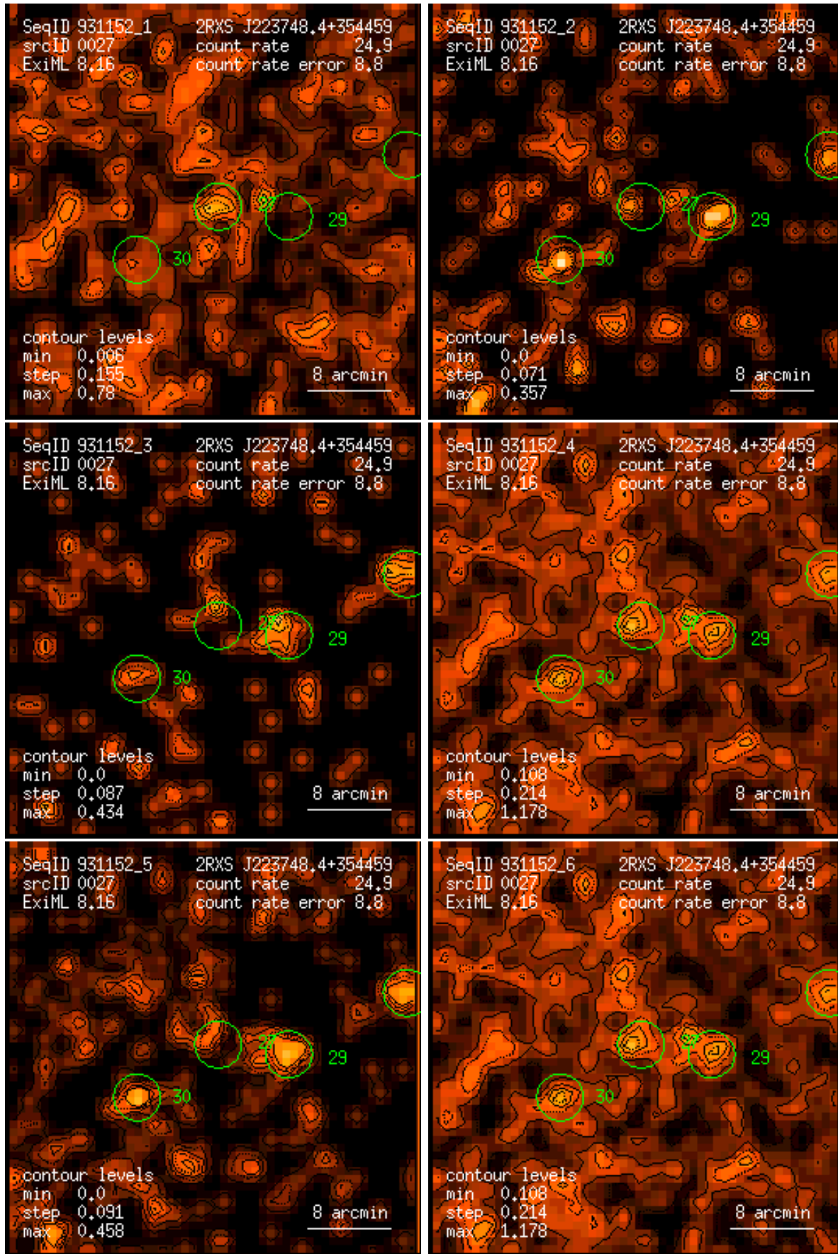
Figure 27: RASS 931152: detection 0027: band rate images, Gaussian filter: (1) PSPC channels 11 – 41, (2) 52 – 90, (3) 91 – 201, (4) 11 – 235, (5) 52 – 201, (6) 11 – 201. Broad band rates in counts/ks. Band rate contour levels in counts/ks/arcmin 2 .
