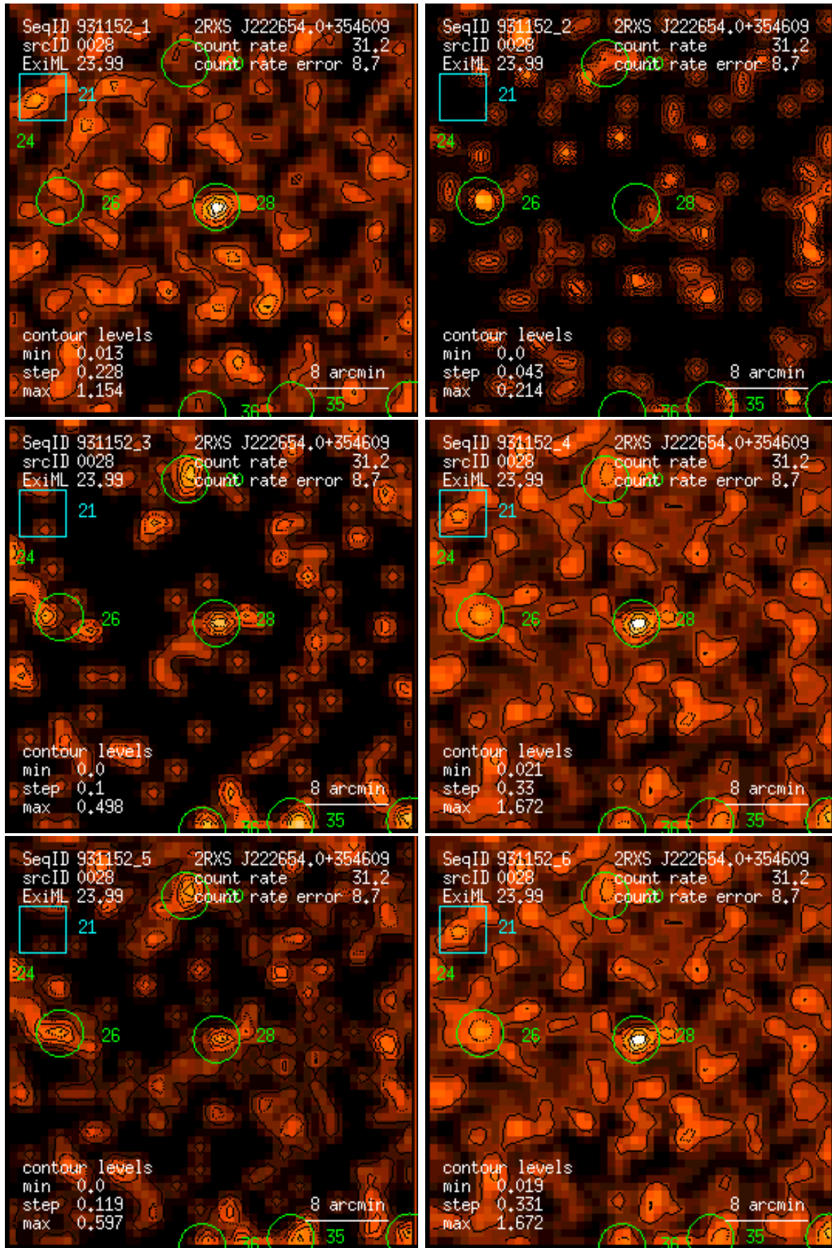
Figure 28: RASS 931152: detection 0028: band rate images, Gaussian filter: (1) PSPC channels 11 – 41, (2) 52 – 90, (3) 91 – 201, (4) 11 – 235, (5) 52 – 201, (6) 11 – 201. Broad band rates in counts/ks. Band rate contour levels in counts/ks/arcmin 2 .
