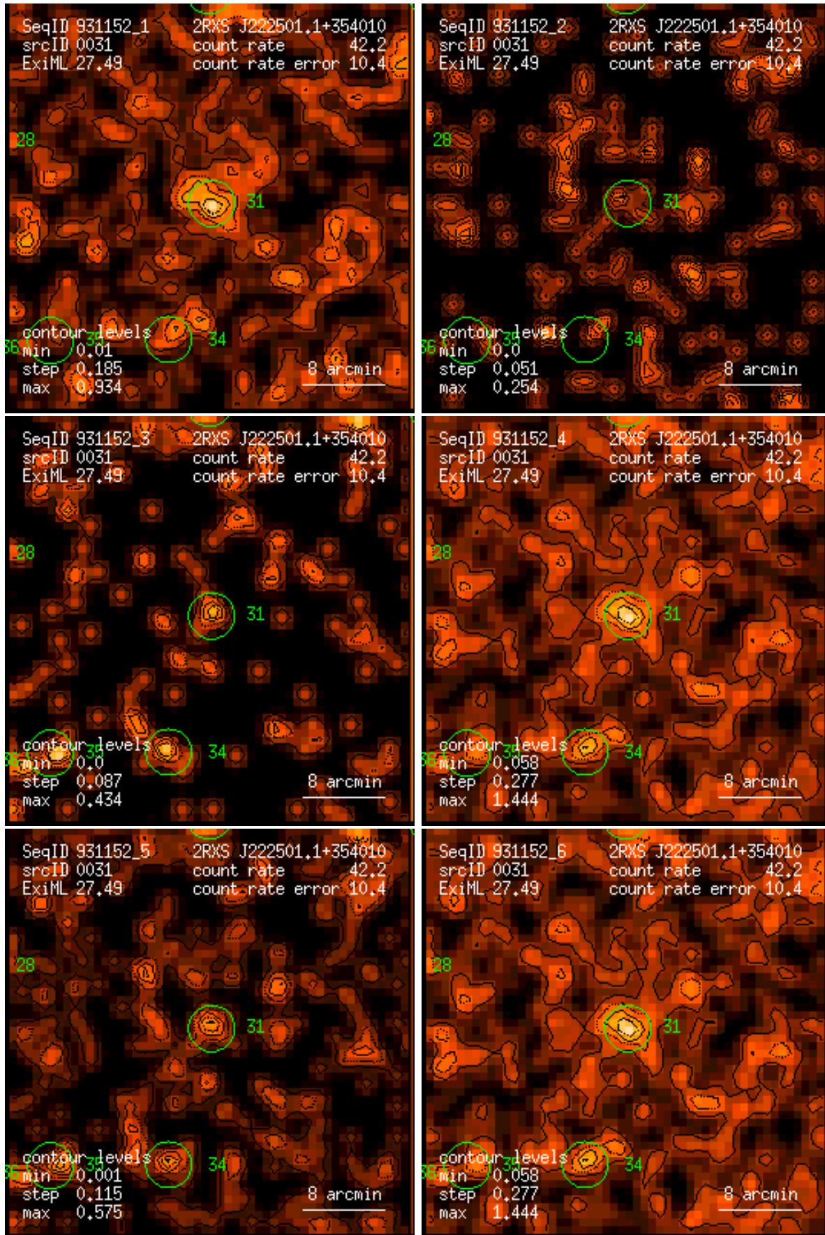
Figure 31: RASS 931152: detection 0031: band rate images, Gaussian filter: (1) PSPC channels 11 – 41, (2) 52 – 90, (3) 91 – 201, (4) 11 – 235, (5) 52 – 201, (6) 11 – 201. Broad band rates in counts/ks. Band rate contour levels in counts/ks/arcmin 2 .
