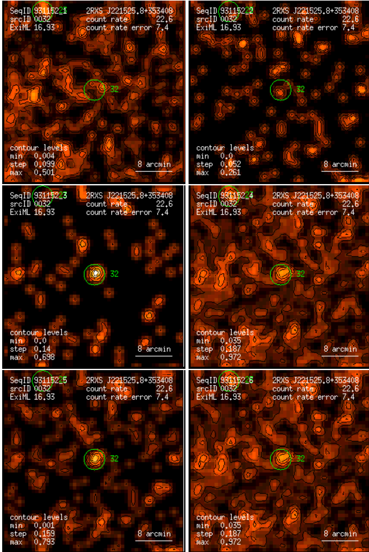
Figure 32: RASS 931152: detection 0032: band rate images, Gaussian filter: (1) PSPC channels 11 – 41, (2) 52 – 90, (3) 91 – 201, (4) 11 – 235, (5) 52 – 201, (6) 11 – 201. Broad band rates in counts/ks. Band rate contour levels in counts/ks/arcmin 2 .
