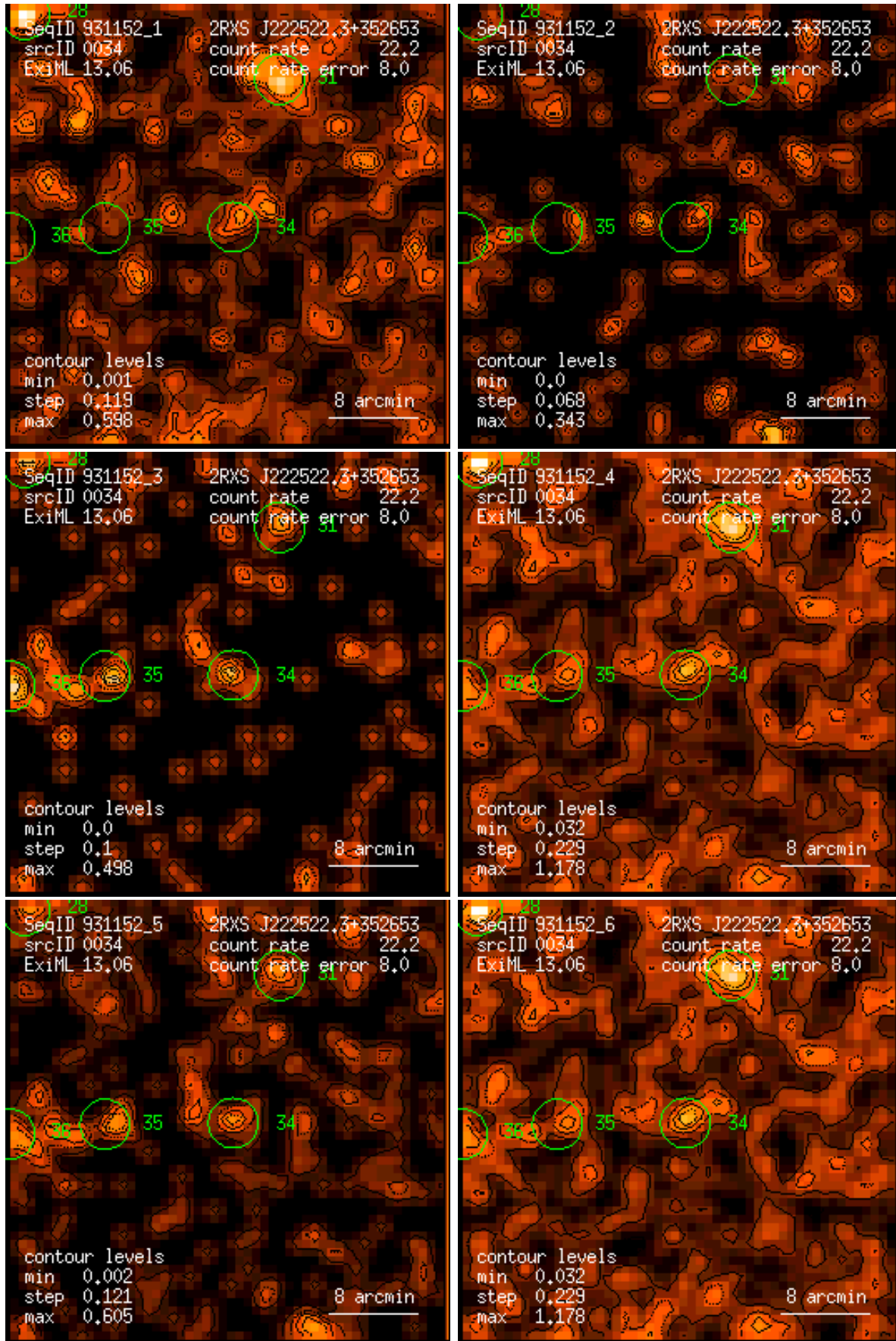
Figure 34: RASS 931152: detection 0034: band rate images, Gaussian filter: (1) PSPC channels 11 – 41, (2) 52 – 90, (3) 91 – 201, (4) 11 – 235, (5) 52 – 201, (6) 11 – 201. Broad band rates in counts/ks. Band rate contour levels in counts/ks/arcmin 2 .
