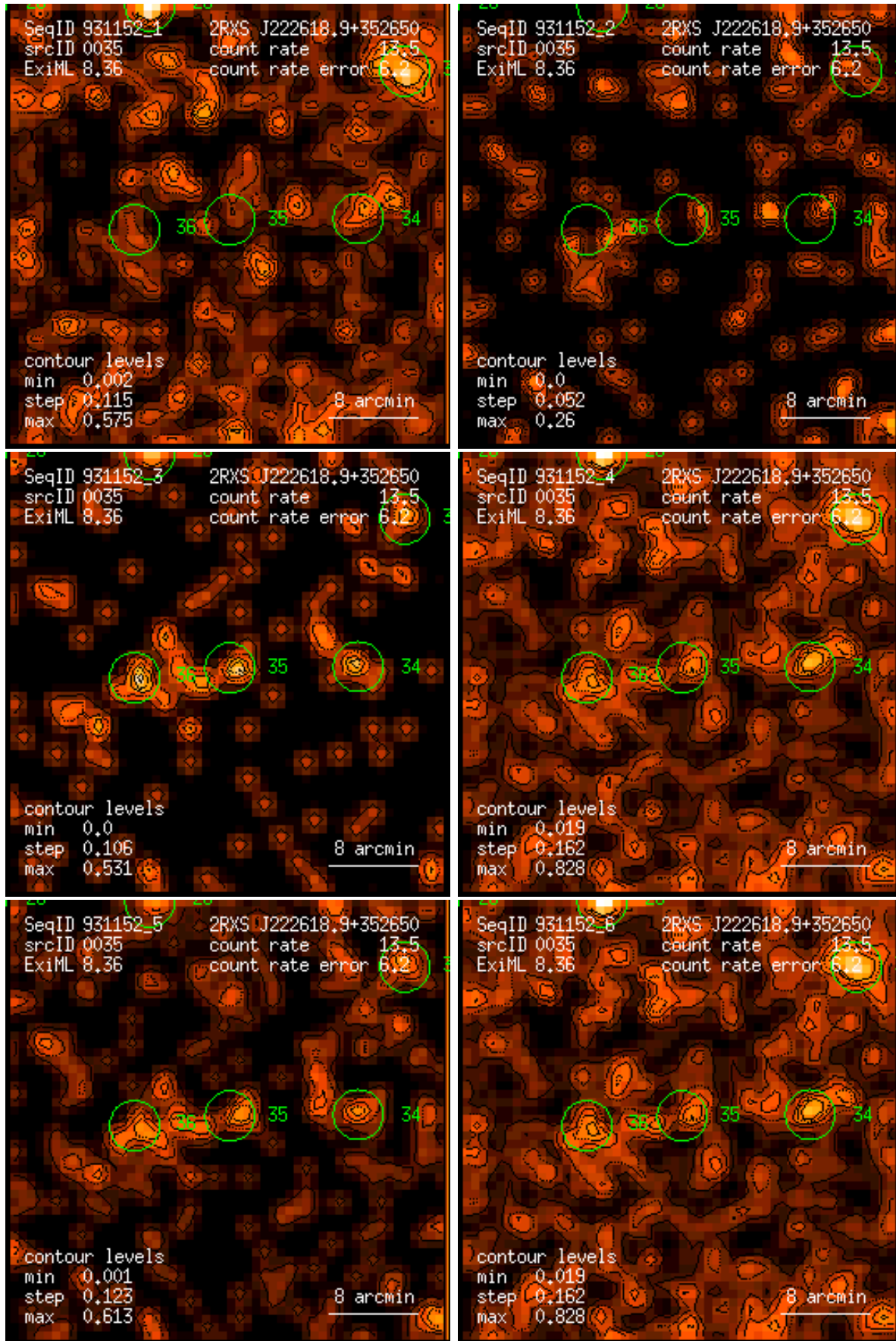
Figure 35: RASS 931152: detection 0035: band rate images, Gaussian filter: (1) PSPC channels 11 – 41, (2) 52 – 90, (3) 91 – 201, (4) 11 – 235, (5) 52 – 201, (6) 11 – 201. Broad band rates in counts/ks. Band rate contour levels in counts/ks/arcmin 2 .
