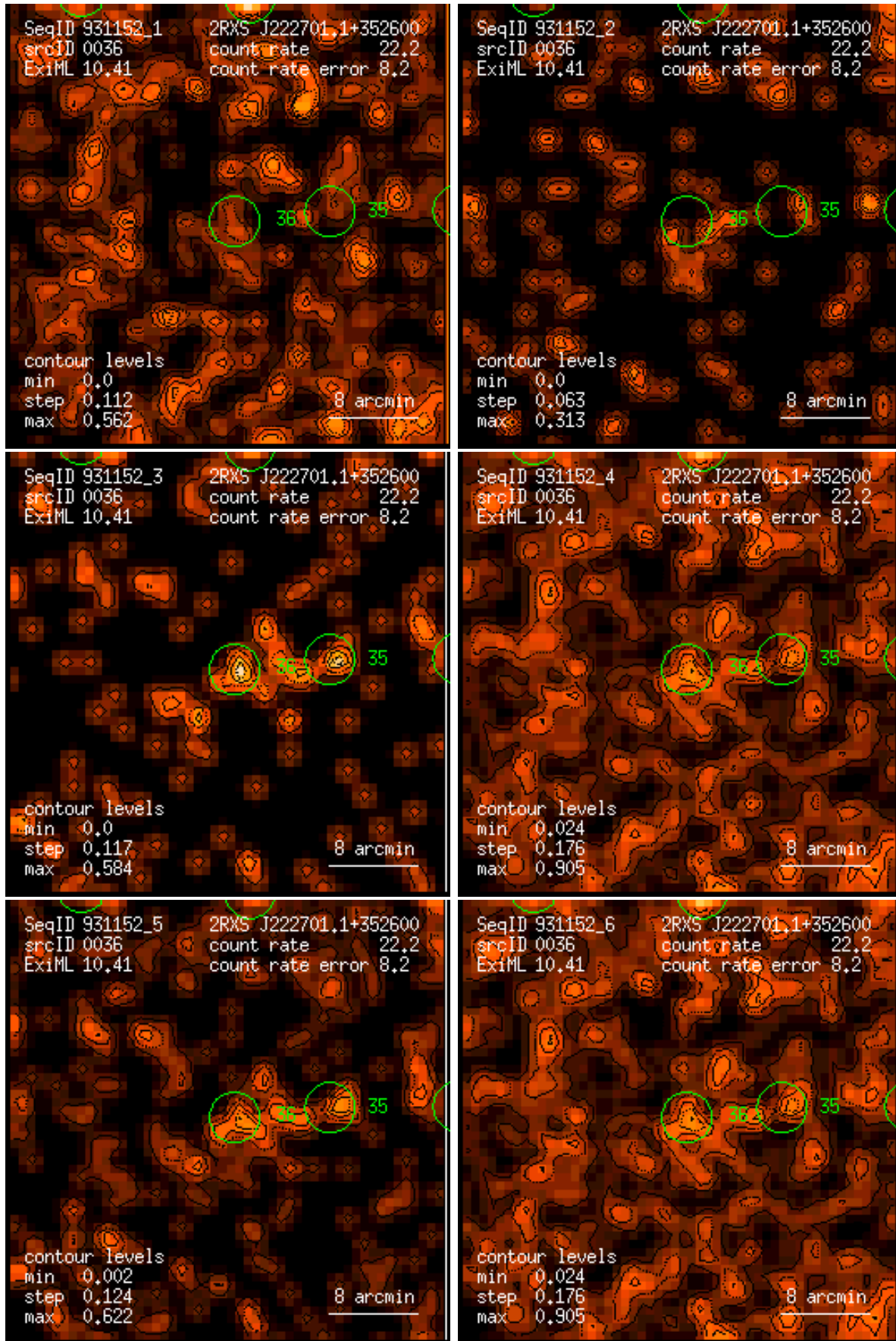
Figure 36: RASS 931152: detection 0036: band rate images, Gaussian filter: (1) PSPC channels 11 – 41, (2) 52 – 90, (3) 91 – 201, (4) 11 – 235, (5) 52 – 201, (6) 11 – 201. Broad band rates in counts/ks. Band rate contour levels in counts/ks/arcmin 2 .
