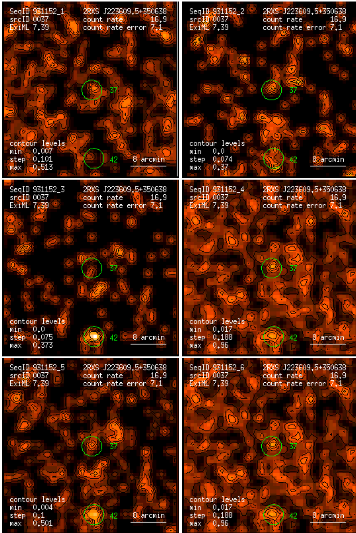
Figure 37: RASS 931152: detection 0037: band rate images, Gaussian filter: (1) PSPC channels 11 – 41, (2) 52 – 90, (3) 91 – 201, (4) 11 – 235, (5) 52 – 201, (6) 11 – 201. Broad band rates in counts/ks. Band rate contour levels in counts/ks/arcmin 2 .
