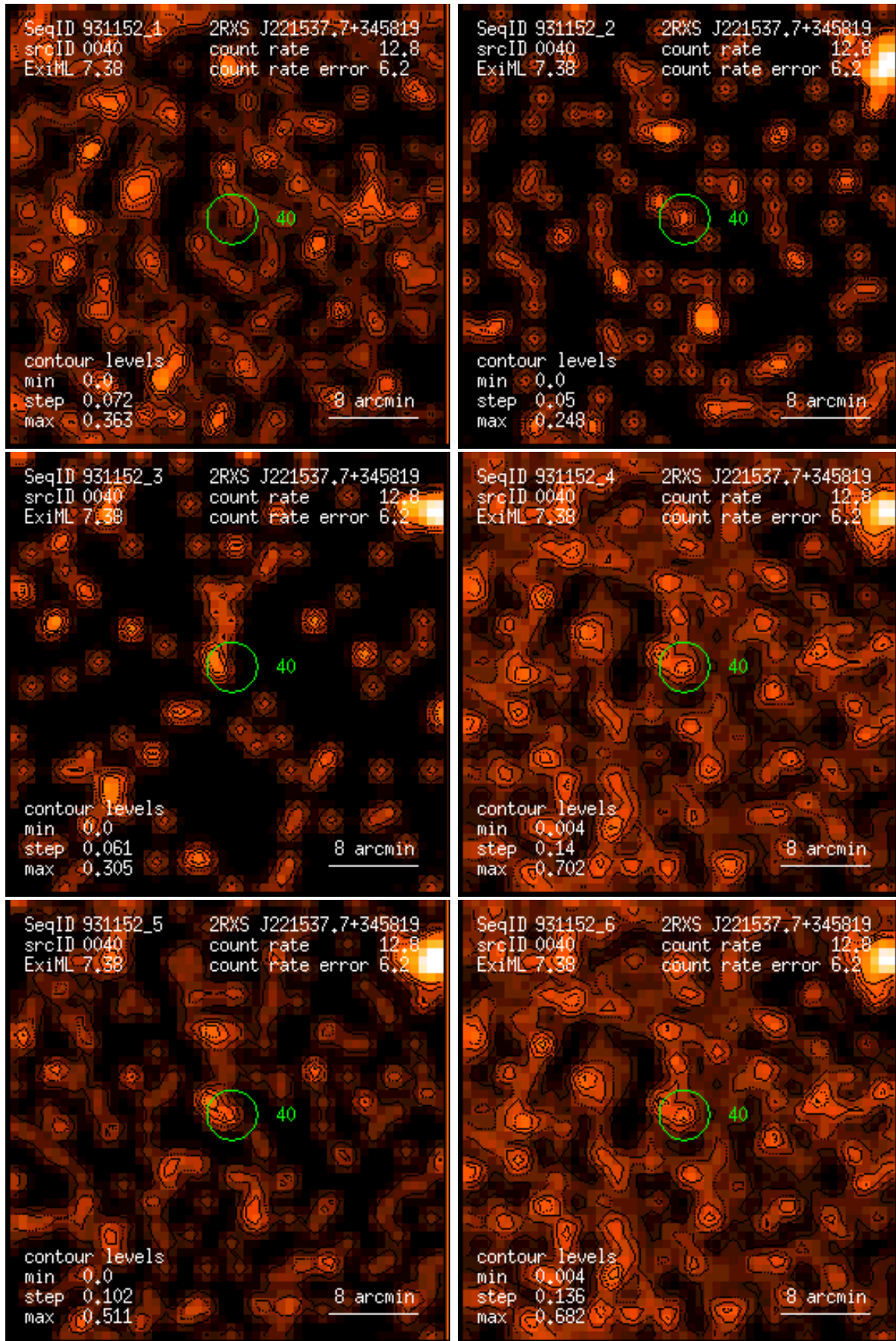
Figure 40: RASS 931152: detection 0040: band rate images, Gaussian filter: (1) PSPC channels 11 – 41, (2) 52 – 90, (3) 91 – 201, (4) 11 – 235, (5) 52 – 201, (6) 11 – 201. Broad band rates in counts/ks. Band rate contour levels in counts/ks/arcmin 2 .
