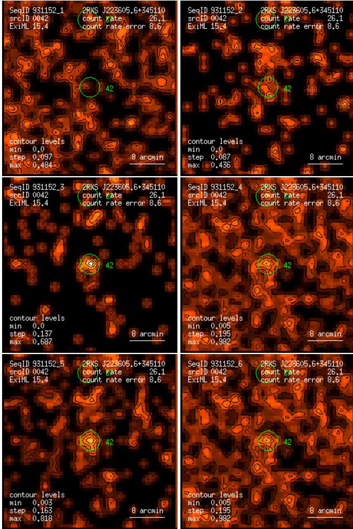
Figure 42: RASS 931152: detection 0042: band rate images, Gaussian filter: (1) PSPC channels 11 – 41, (2) 52 – 90, (3) 91 – 201, (4) 11 – 235, (5) 52 – 201, (6) 11 – 201. Broad band rates in counts/ks. Band rate contour levels in counts/ks/arcmin 2 .
