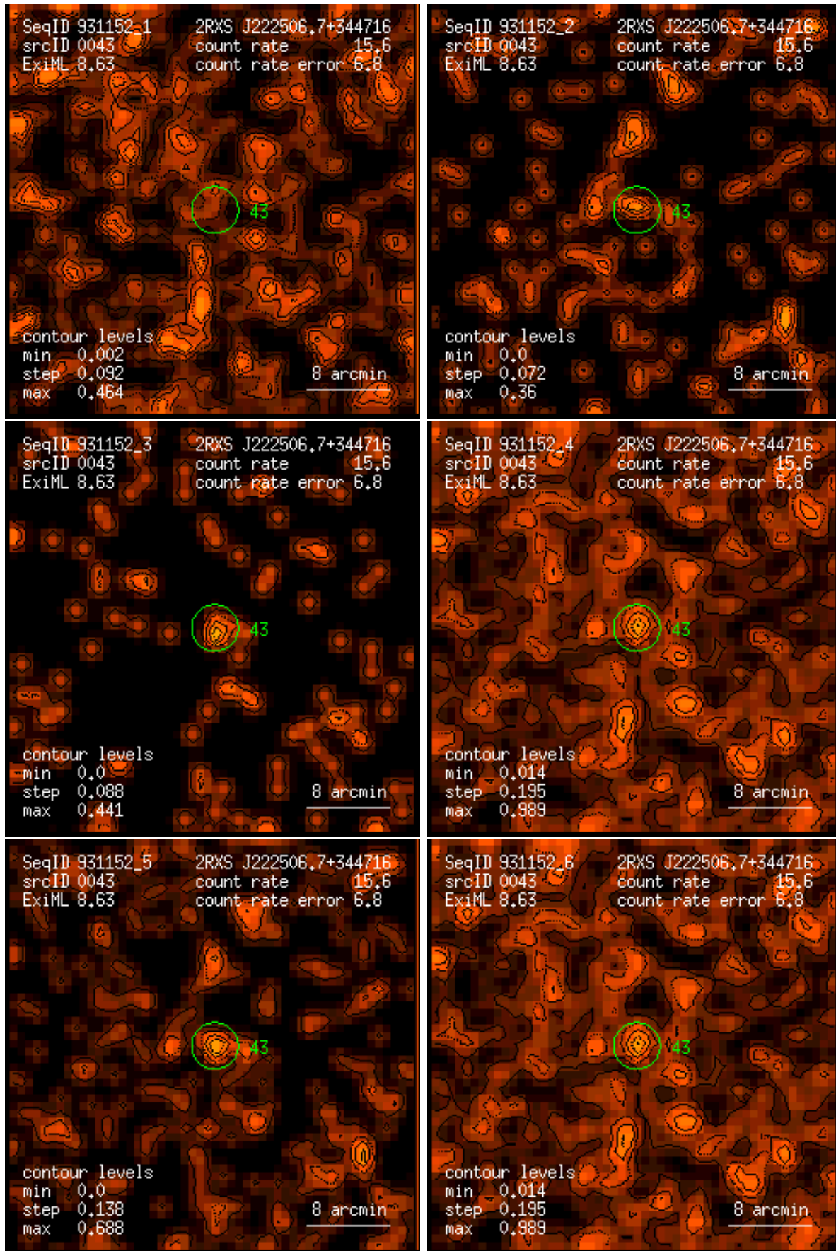
Figure 43: RASS 931152: detection 0043: band rate images, Gaussian filter: (1) PSPC channels 11 – 41, (2) 52 – 90, (3) 91 – 201, (4) 11 – 235, (5) 52 – 201, (6) 11 – 201. Broad band rates in counts/ks. Band rate contour levels in counts/ks/arcmin 2 .
