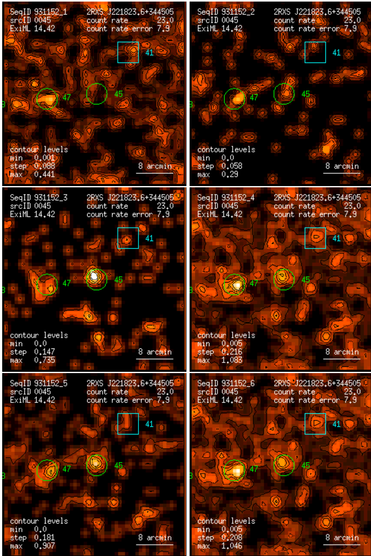
Figure 45: RASS 931152: detection 0045: band rate images, Gaussian filter: (1) PSPC channels 11 – 41, (2) 52 – 90, (3) 91 – 201, (4) 11 – 235, (5) 52 – 201, (6) 11 – 201. Broad band rates in counts/ks. Band rate contour levels in counts/ks/arcmin 2 .
