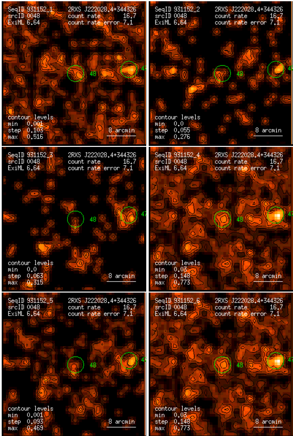
Figure 48: RASS 931152: detection 0048: band rate images, Gaussian filter: (1) PSPC channels 11 – 41, (2) 52 – 90, (3) 91 – 201, (4) 11 – 235, (5) 52 – 201, (6) 11 – 201. Broad band rates in counts/ks. Band rate contour levels in counts/ks/arcmin 2 .
